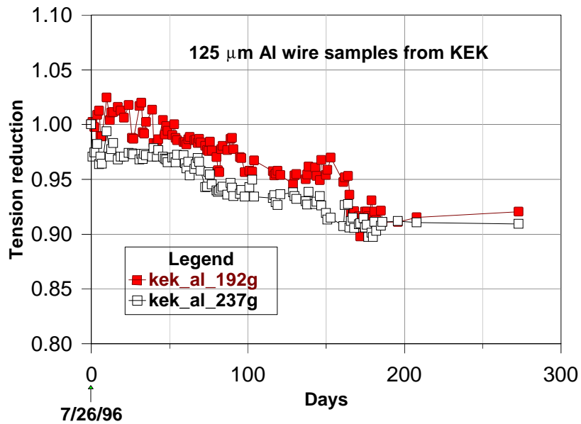
Figure 5: KEK bare aluminum wire, 125 \mu\text{m} .
