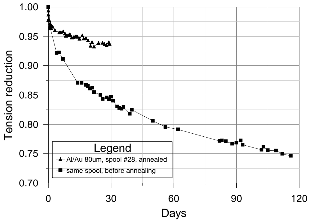
Figure 1: Comparison of spool 28 of the CFW 80- \mu m wire delivered in Dec. 1996, before and after annealing. See also, Princeton/BABAR/TNDC-97-56.
