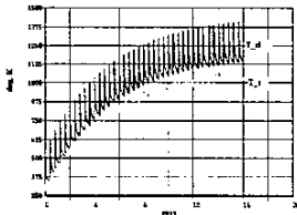
Figure 3: Transient temperatures in the C-C target
