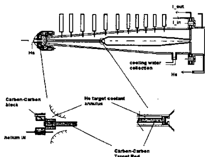
Figure 1: Horn/Target Configuration
