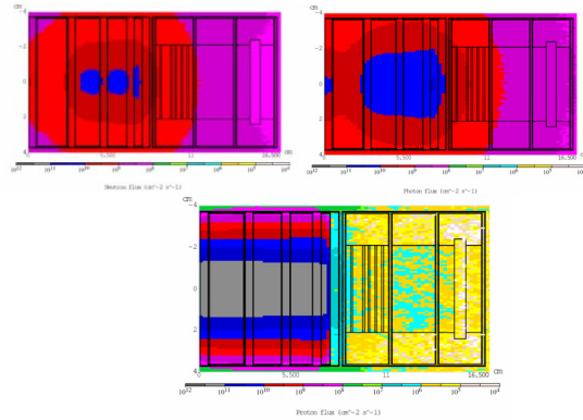
Figure 6: Estimated neutron, photon and proton spectra in the target irradiation arrangement (MARS15 code)
