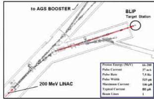
Figure 2: Schematic of the BNL BLIP irradiation facility
