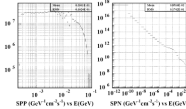
Figure 7: Estimated proton and neutron energy spectra
