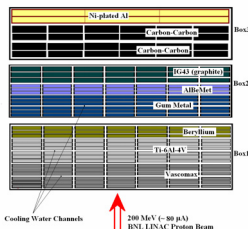
Figure 3: Target assembly for 200 MeV proton irradiation
