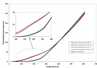
Figure 11: Damage reversal or CTE restoration in super-Invar following a second, higher dose proton irradiation
