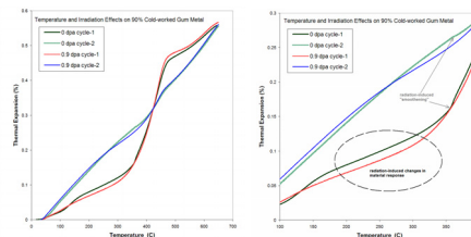
Figure 14: Proton irradiation and thermal effects on gum
