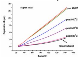
Figure 10: Damage reversal or CTE restoration in irradiated super Invar through thermal annealing
