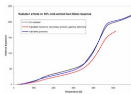
Figure 15: Proton and neutron irradiation effect comparison on the thermal expansion of gum metal
