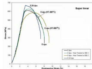
Figure 9: Proton irradiation effects and temperature effects on the stress-strain relation of super-Invar
