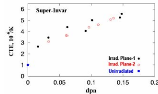
Figure 8: Proton irradiation effects on super-Invar CTE
