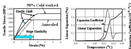
Figure 1: Un-irradiated Gum material properties [4]
