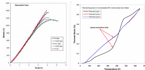
Figure 13: Irradiation-induced ductility loss and thermal cycle effects on Gum metal
