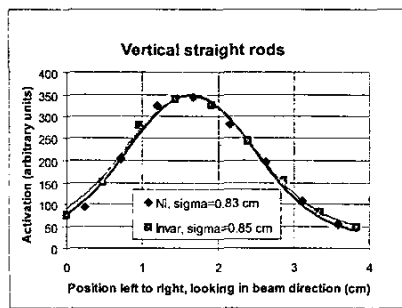
Figure 2: Measured specimen activity as a function of target position. The lines are Gaussian fits.
