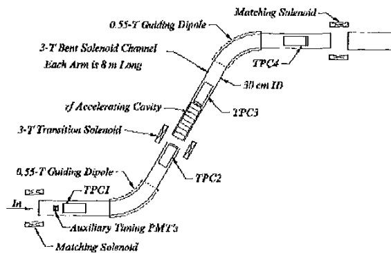
Figure 1: Schematic of the measurement channel
