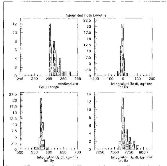
Figure 5: a : Total path length from TPC1 to TPC2; b : \int B_x dx c : \int B_y dy , d : \int B_z dz
