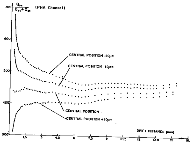
Figure 14: Measurement of the transverse coordinate as a function of the drift distance.
