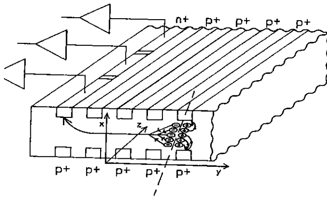
Figure 1: Perspective view (not to scale) of a semiconductor drift detector. Electrons created by an ionizing particle are transported long distances parallel to the detector surface. The anode is divided into short segments to measure the coordinate perpendicular to the drift direction.
