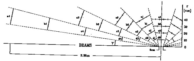
Figure 15: Cross section along the beam axis of the inner tracking detector based on silicon drift detectors. Detector has a full azimuthal coverage and rapidity coverage |\eta| \leq 3 . Lines indicate the cross section of rings of detectors centered around the beam axis. Each line represents close layers of silicon drift detectors.
