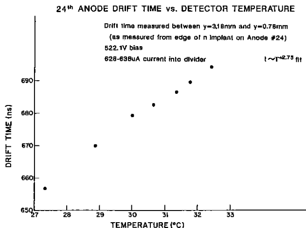
Figure 9: Drift time for 2.4mm drift distance as a function of the detector temperature.
