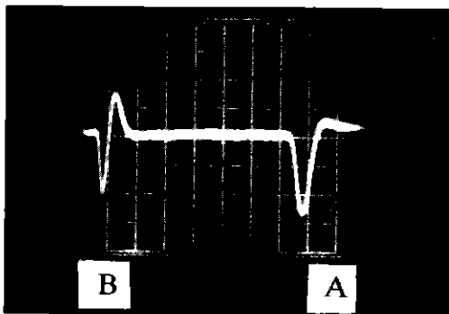
Figure 7: A-pulse corresponding to the collection of the injected charge after an electron drift time of 3.8\mu s . B-injection start pulse.
