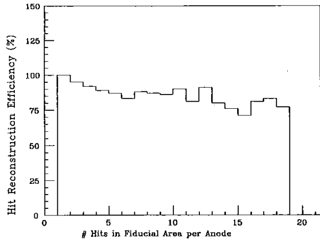
Figure 22: The efficiency for identifying and fitting a hit signal in the presence of other pileup hits is shown. Here the method of identifying a hit uses a center of gravity calculation about a peak, and subtraction according to the known amplitude for a minimum ionizing hit.
