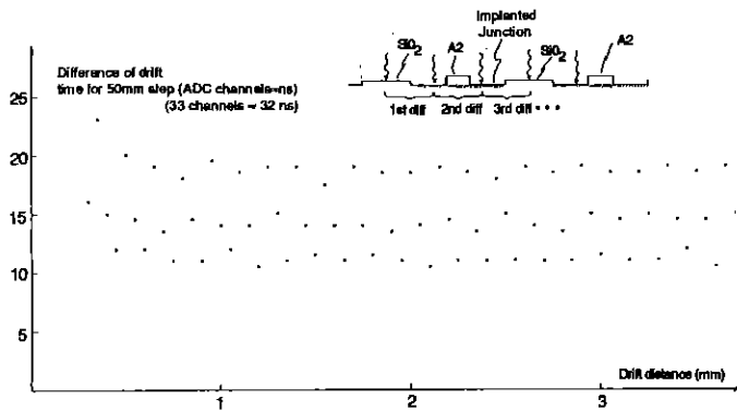
Figure 12: Drift time differences for 50\mu\text{m} steps along the drift direction.
