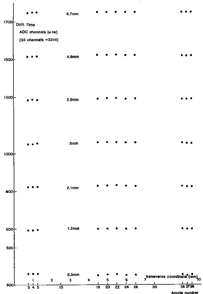
Figure 13: Drift time as a function of the transverse coordinate for several drift distances.
