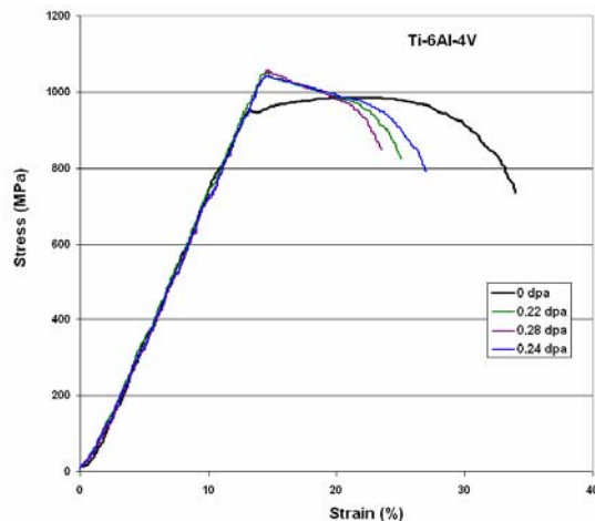
Figure 21: Irradiation effects on stress-strain relation of Ti-6Al-4V
