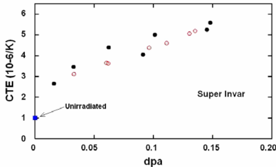
Figure 11: Irradiation effects on the thermal expansion coefficient of super Invar.
