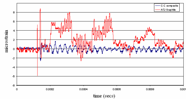
Figure 5: Response to intense beam comparison between graphite and carbon-composite targets
