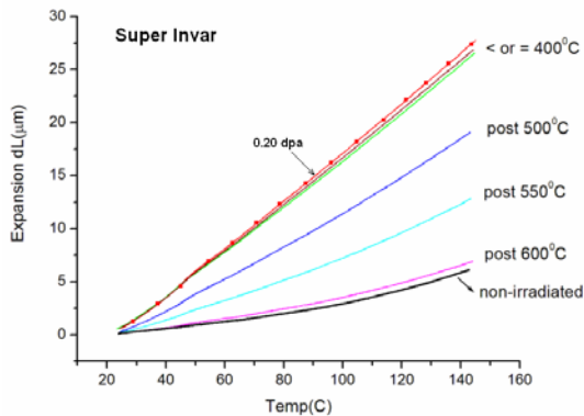
Figure 12: Damage reversal exhibited by the super-Invar alloy during thermal cycling.
