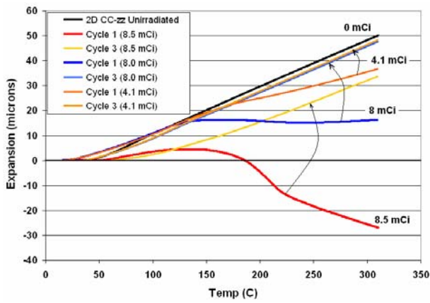
Figure 15: "Annealing" behavior of 2D carbon composite along the normal to fiber-reinforced planes while at different levels of irradiation exposure (expressed in mCi)
