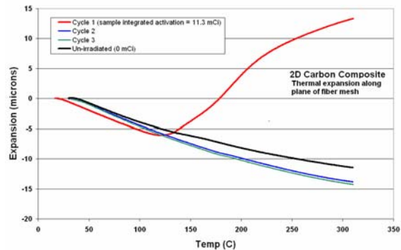
Figure 14: “Annealing” behavior of the 2D carbon-carbon composite (along plane of reinforcing fibers)
