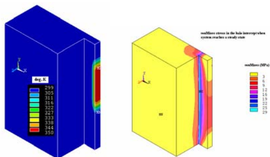
Figure 7: Estimated temperatures and critical stresses in the SNS primary collimator during a full beam intercept
