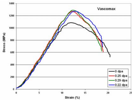
Figure 20: Irradiation effects on the stress-strain relation of Vascomax
