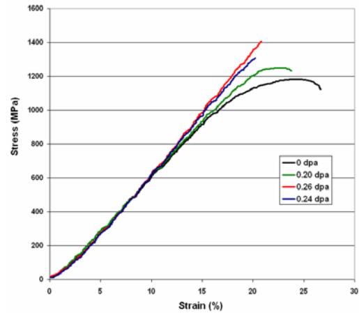
Figure 18: Irradiation effects on the stress-strain behavior of "gum metal"
