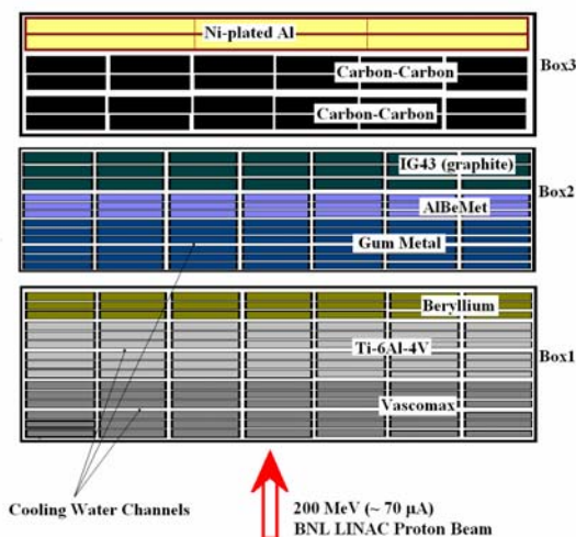
Figure 9: Material matrix arrangement during one of the proton irradiation exposure studies at BNL
