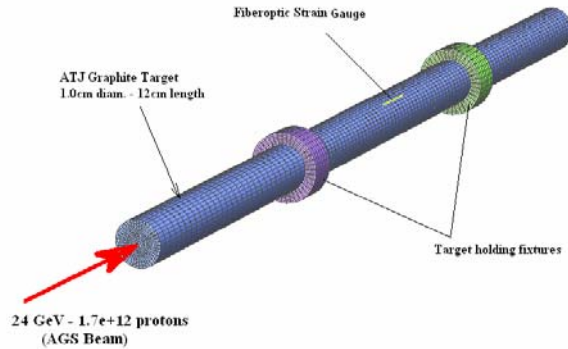
Figure 4: BNL solid target test set-up and instrumentation
