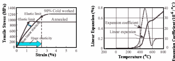
Figure 17: Mechanical and physical properties of the super alloy "gum metal" [Ref. 4]
