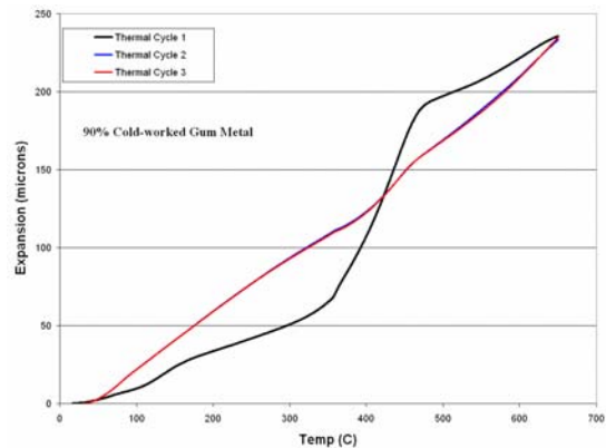
Figure 19: Annealing effects on the cold-worked "Gum metal" thermal expansion
