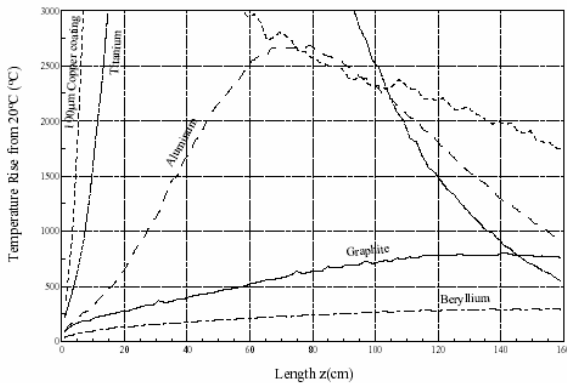
Figure 3: Estimates of temperature in the LHC collimators based on different material choices [Ref. 5]
