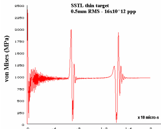
Figure 1: Stress predictions in a stainless steel target intercepting a 16 TP, 100ns proton pulse
