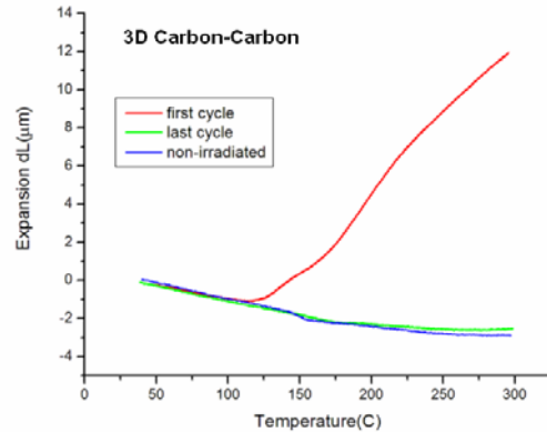
Figure 13: “Annealing” behavior exhibited by the 3D carbon-carbon composite
