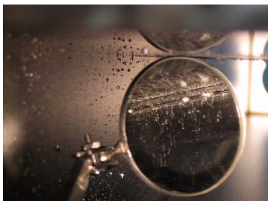
Figure 8: Collimator accident condition following beam miss steering at the FNAL Tevatron
