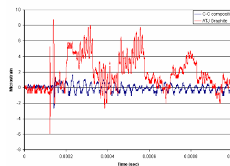
Figure 5: Experimental strains (CC vs. ATJ graphite)
