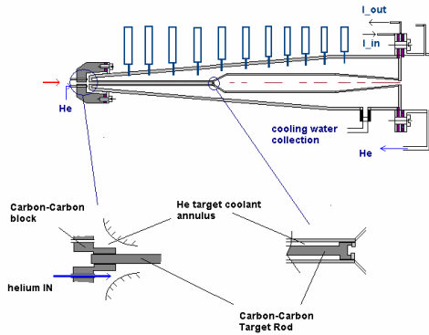
Figure 1: Horn/Target Configuration
