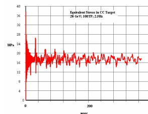
Figure 4: Beam-induced von Mises stresses on target
