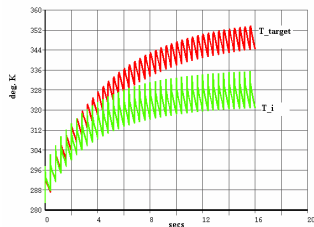
Figure 2: Transient temperatures in the horn conductor
