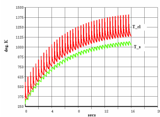
Figure 3: Transient temperatures in the C-C target
