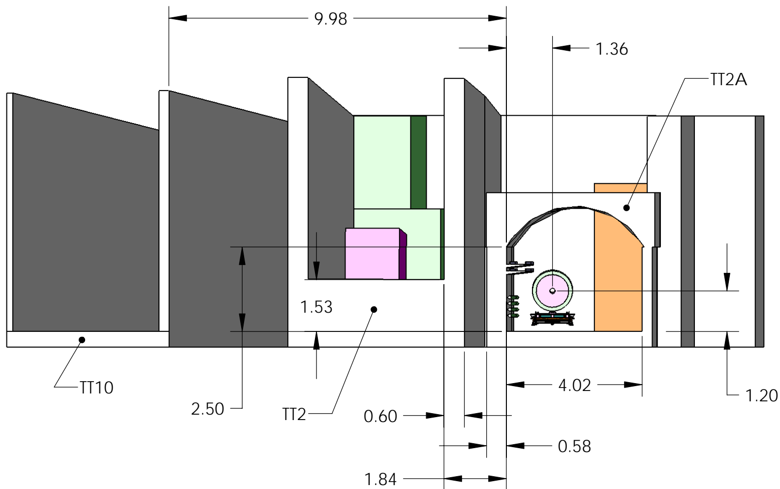
SECTION CUT THROUGH Z=0 NORMAL TO BEAM (MAGNET CENTER 14.8m FROM TT2A CORNER)
