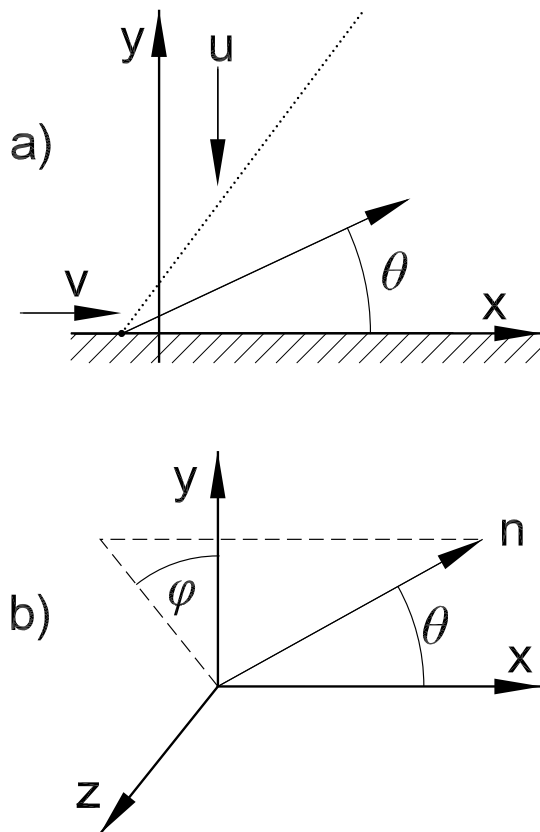
Figure 1: a) A sloping line of charge moves in the -y direction with velocity v_y = u \ll c such that its intercept with the x axis moves with velocity v_x = v > c . As the charge disappears into the conductor at y < 0 it emits transition radiation. The radiation appears to emanate from a spot moving at superluminal velocity and is concentrated on a cone of angle \cos^{-1}(c/v) . b) The angular distribution of the radiation is discussed in a spherical coordinates system about the x axis.
