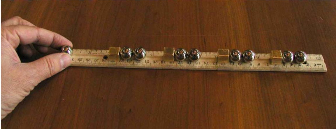
Figure 1: The magnetic linear accelerator, from Scitoys.com [1]
