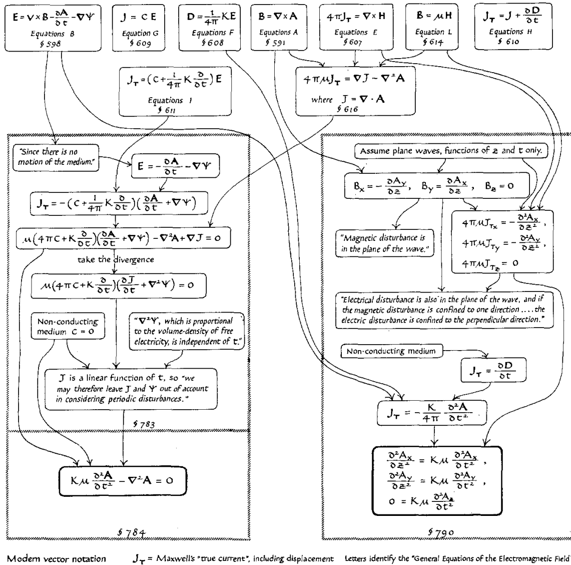
Figure 5: Flow chart of Maxwell's derivation of the electromagnetic wave equations in [19]. From Fig. 3 of [6].
