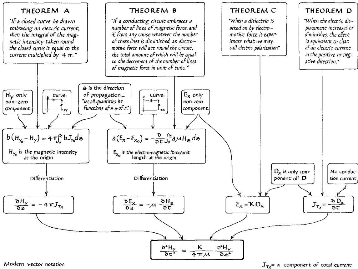
Figure 4: Flow chart of Maxwell's derivation of the electromagnetic wave equation in [26]. From Fig. 2 of [6].
