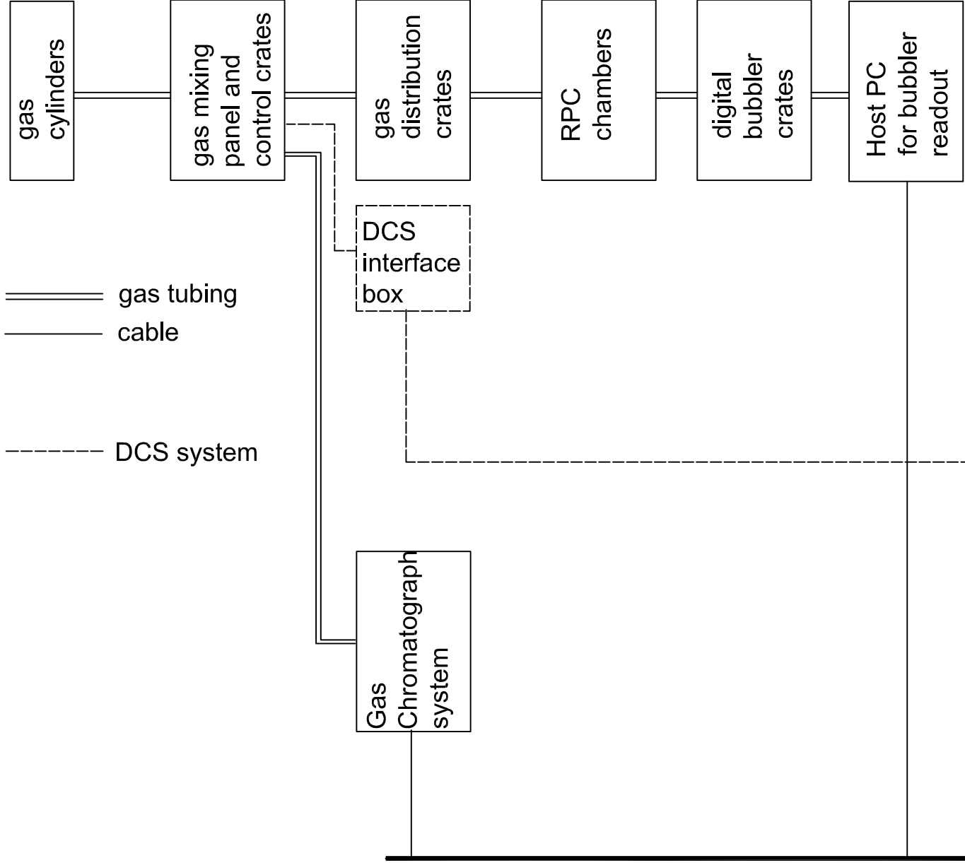
RPC gas system in Daya Bay Near Hall
