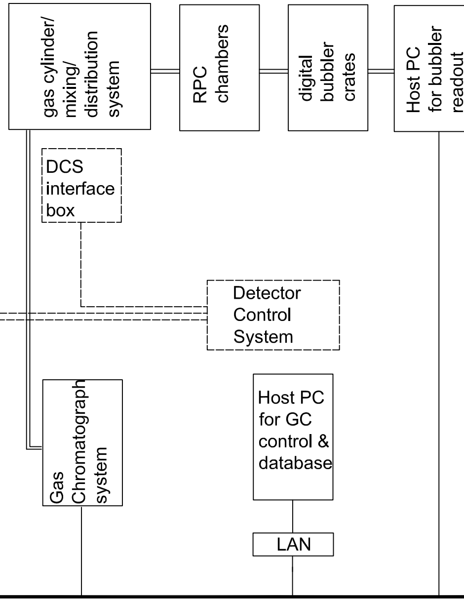
RPC gas system in Daya Bay Far Hall
