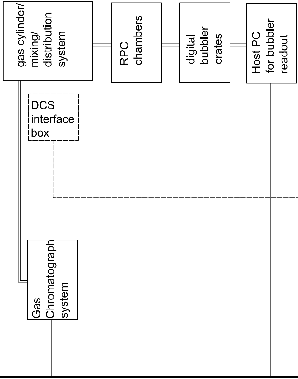
RPC gas system in Linao Near Hall
