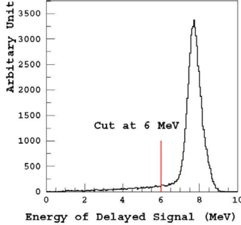
Fig. 2.4. GEANT3 simulation of the spectrum of the energy of \gamma 's from the capture of a thermal neutron by a Gd nucleus. The simulation includes a detector module with 200 PMT's and 20 tons of Gd-loaded liquid scintillator surrounded by a 45-cm thick \gamma -catcher.
