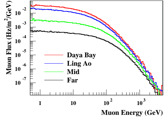
Fig. 2.7. Muon flux as a function of the energy of the surviving muons. The four curves from upper to lower corresponds to the Daya Bay near site, the Ling Ao near site, the mid site and the far site, respectively.
