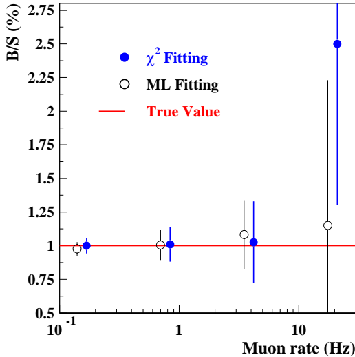
Fig. 2.9. Fitting results as a function of the muon rate. The error bars show the precision of the fitting. The \chi^2 fitting uses the same muon rate as ML fitting but shown on the right of it.
