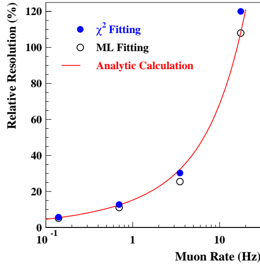
Fig. 2.10. The fitting precision as a function of the muon rate, comparing with the analytic estimation of Eq. 32. The y-axis shows the relative resolution of the background-to-signal ratio.
