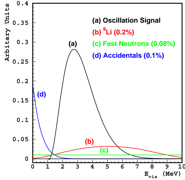
Fig. 2.12. Spectra of three major backgrounds for the Daya Bay experiment and their size relative to the oscillation signal.
