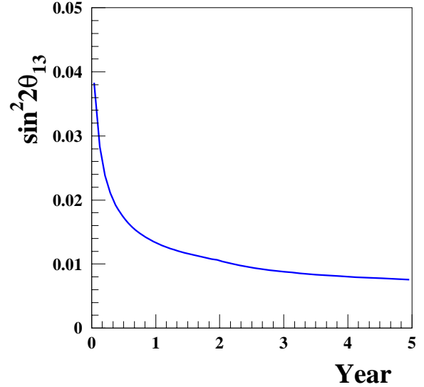
Fig. 2.14. Expected \sin^2 2\theta_{13} sensitivity at 90% C.L. versus year of data taking of the full measurement, with two near sites and one far site. The \Delta m^2 is taken to be 2.5 \times 10^{-3} \text{ eV}^2 .
