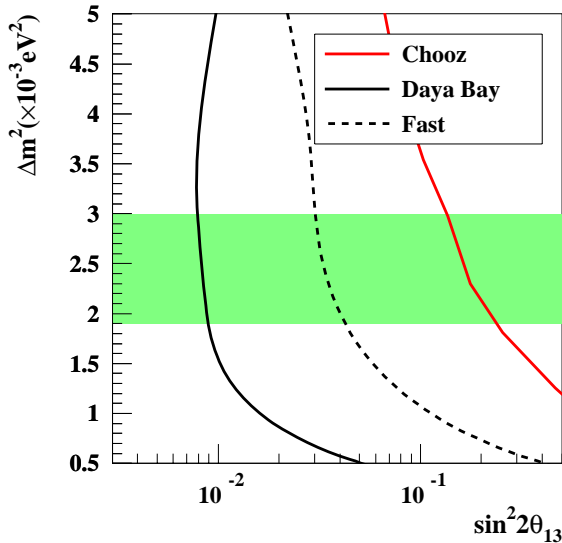
Fig. 2.13. Expected \sin^2 2\theta_{13} sensitivity at 90% C.L. with 3 years of data, as shown in solid black line. The dashed line shows the sensitivity of the fast measurement with the DYB near site and the mid site only. The red line shows current upper limit measured by Chooz.
