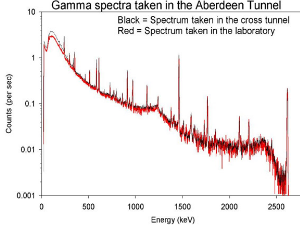
Fig. 2.11. Spectrum of natural radioactivity measured with a Ge crystal in the Hong Kong Aberdeen Tunnel.
