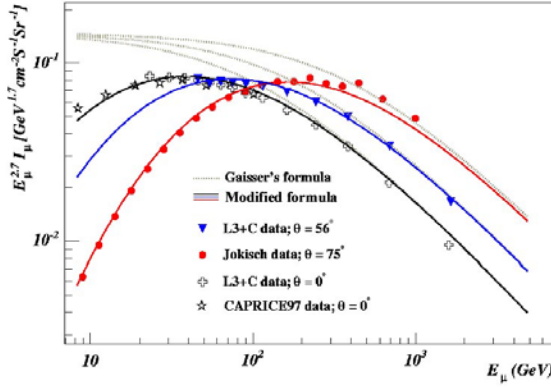
Fig. 2.6. Comparison of the modified formula (solid lines) with data. Calculations with the standard Gaisser's formula are shown in dashed lines. The data are taken from Ref.[4,5].
