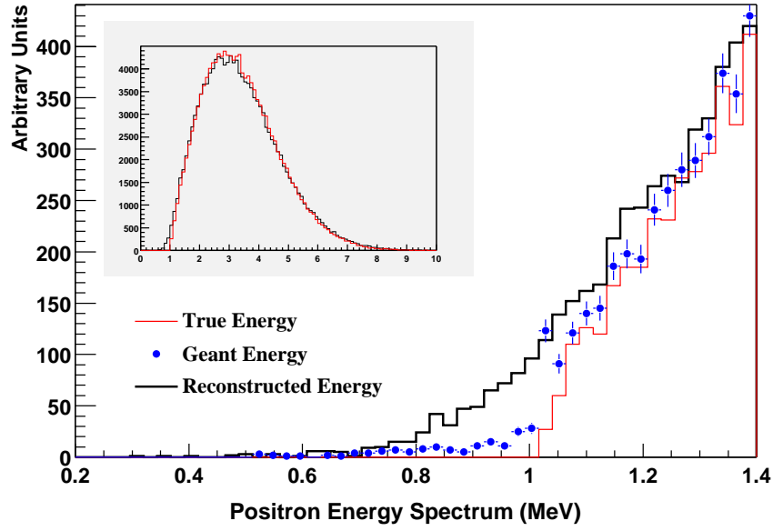
Fig. 2.3. Spectra of the energy of positrons from antineutrino interactions for true, simulated (GEANT), and reconstructed energy at around 1 MeV. The full spectrum is shown in the inset, where the red line corresponds to the true energy and the black one corresponds to the reconstructed energy.
