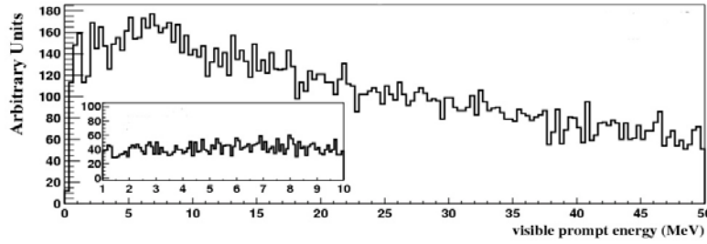
Fig. 2.8. The prompt energy spectrum of fast neutron backgrounds at the Daya Bay far detector. The inset is an expanded view of the spectrum from 1 to 10 MeV.
