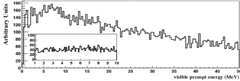
Fig. 2.7. The prompt energy spectrum of fast neutron backgrounds at the Daya Bay far detector. The inset is an expanded view of the spectrum from 1 to 10 MeV.
