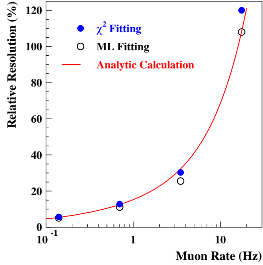
Fig. 2.9. The fitting precision as a function of the muon rate, comparing with the analytic estimation of Eq. 33. The y-axis shows the relative resolution of the background-to-signal ratio.
