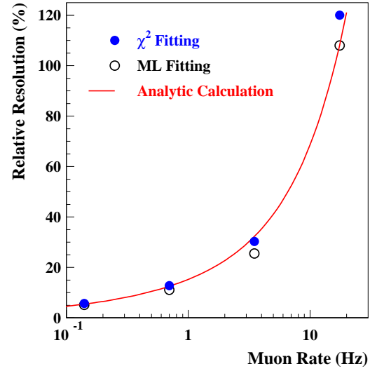
Fig. 3.10. The fitting precision as a function of the muon rate, comparing with the analytic estimation of Eq. 33. The y-axis shows the relative resolution of the background-to-signal ratio.
