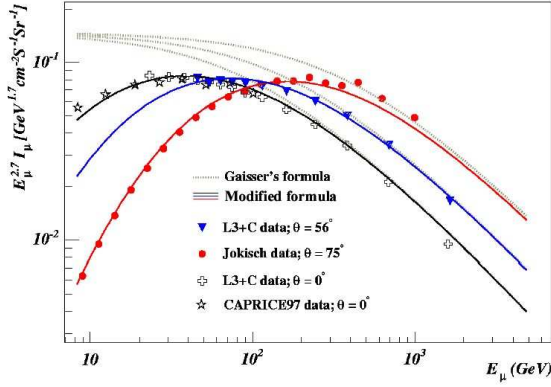
Fig. 3.6. Comparison of the modified formula (solid lines) with data. Calculations with the standard Gaisser's formula are shown in dashed lines. The data are taken from Ref.[4,5].
