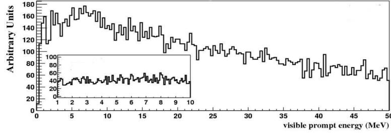
Fig. 3.8. The prompt energy spectrum of fast neutron backgrounds at the Daya Bay far detector. The inset is an expanded view of the spectrum from 1 to 10 MeV.
