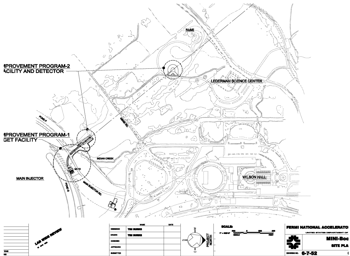
Figure 2.2: The MiniBooNE local site plan, showing the location of the 8 GeV Fixed Target Facility and the MiniBooNE Target Facility and Detector.
