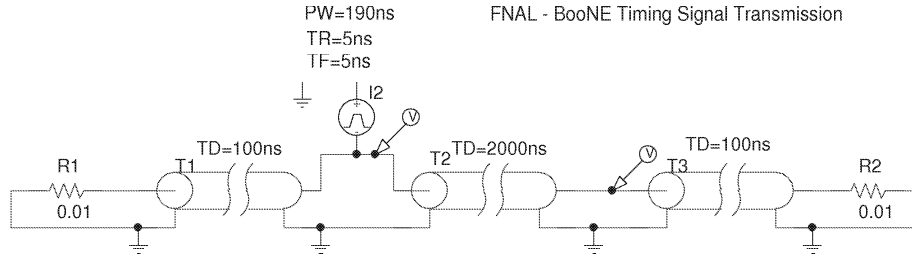
Figure 6.23: schematic of the SPICE simulation.
