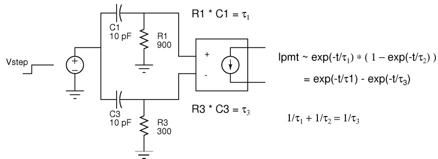
PMT Anode Waveform SPICE Model
