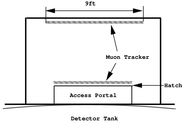
Figure 5.1: Muon tracker
