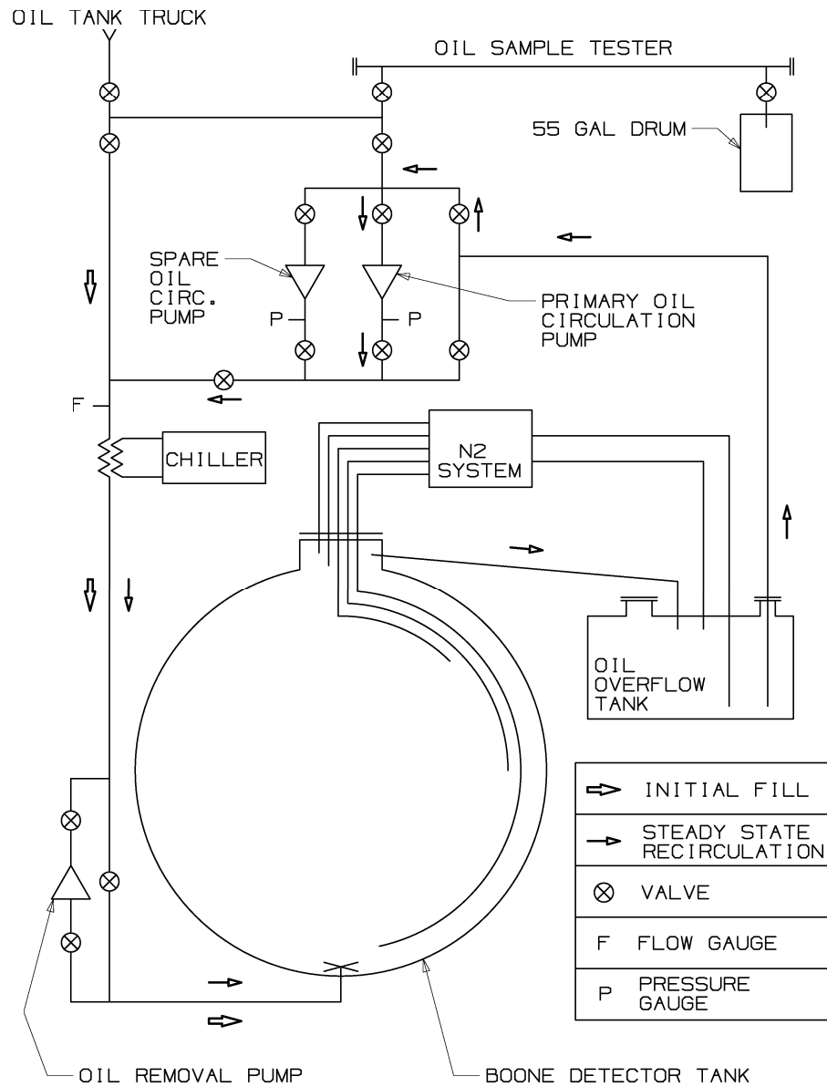
Figure 3.13: A schematic figure showing the oil plumbing scheme.
