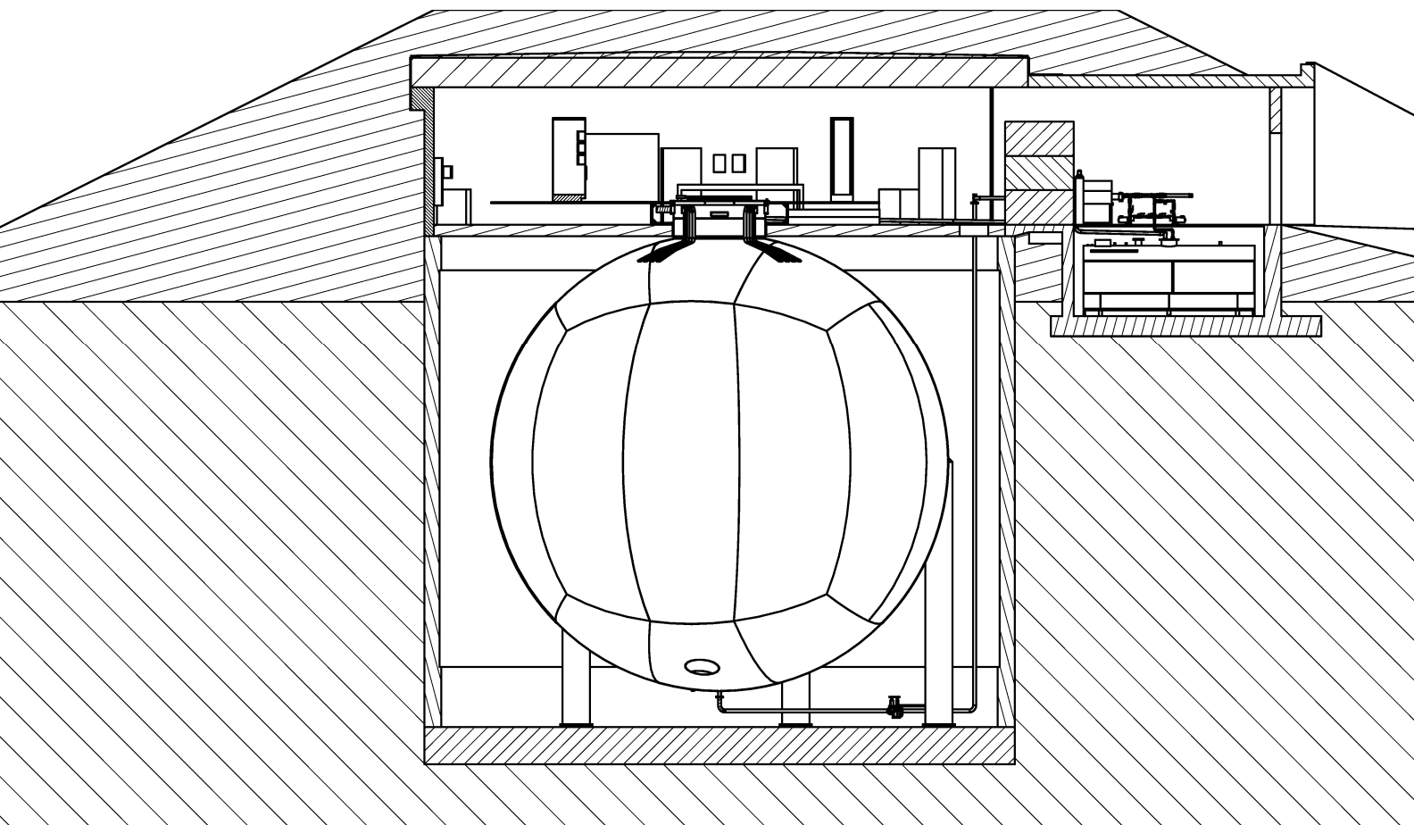
Figure 3.3: The Detector Containment Plant.
