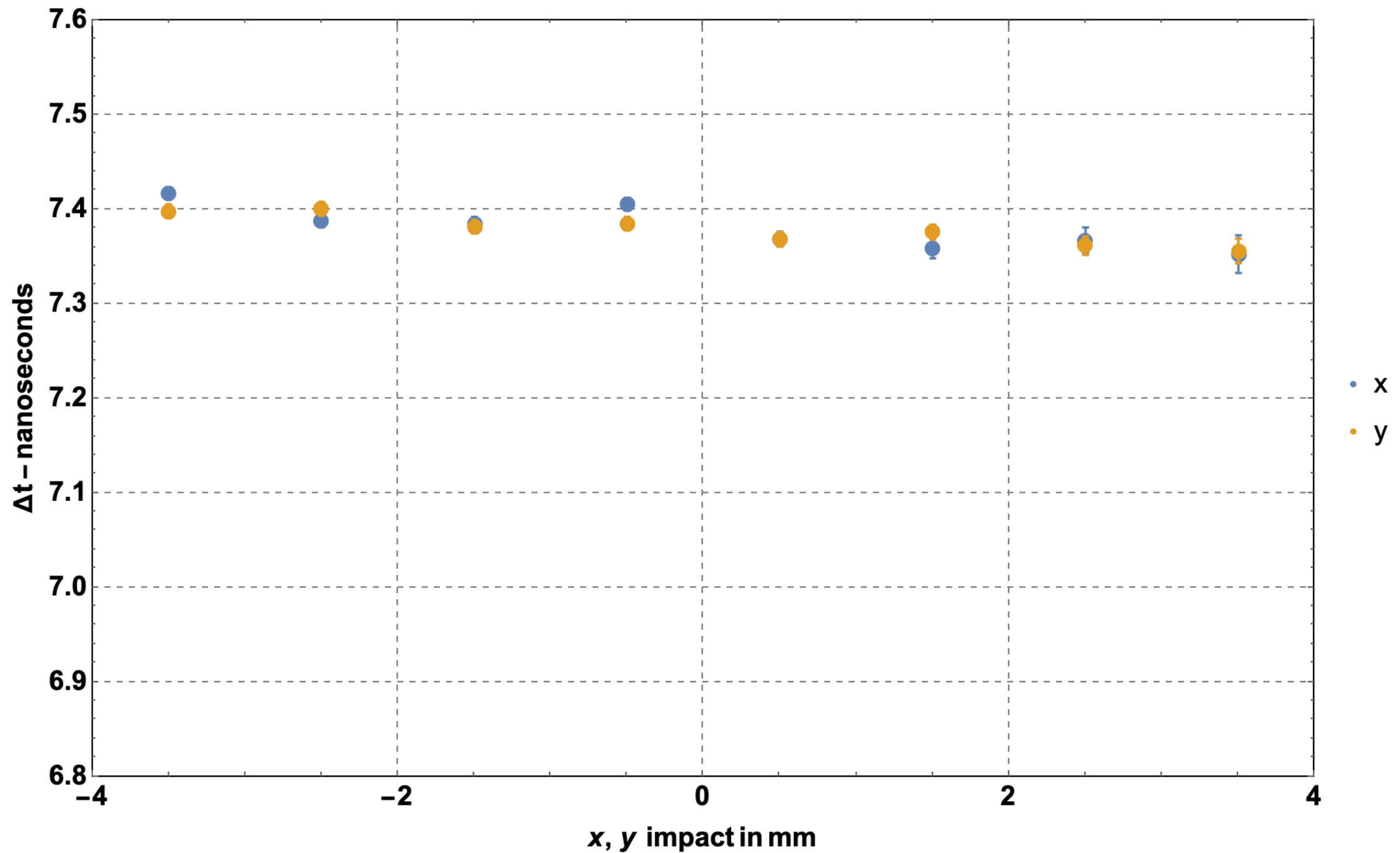
HFS – MCP time vs Impact 150 GeV Muons
