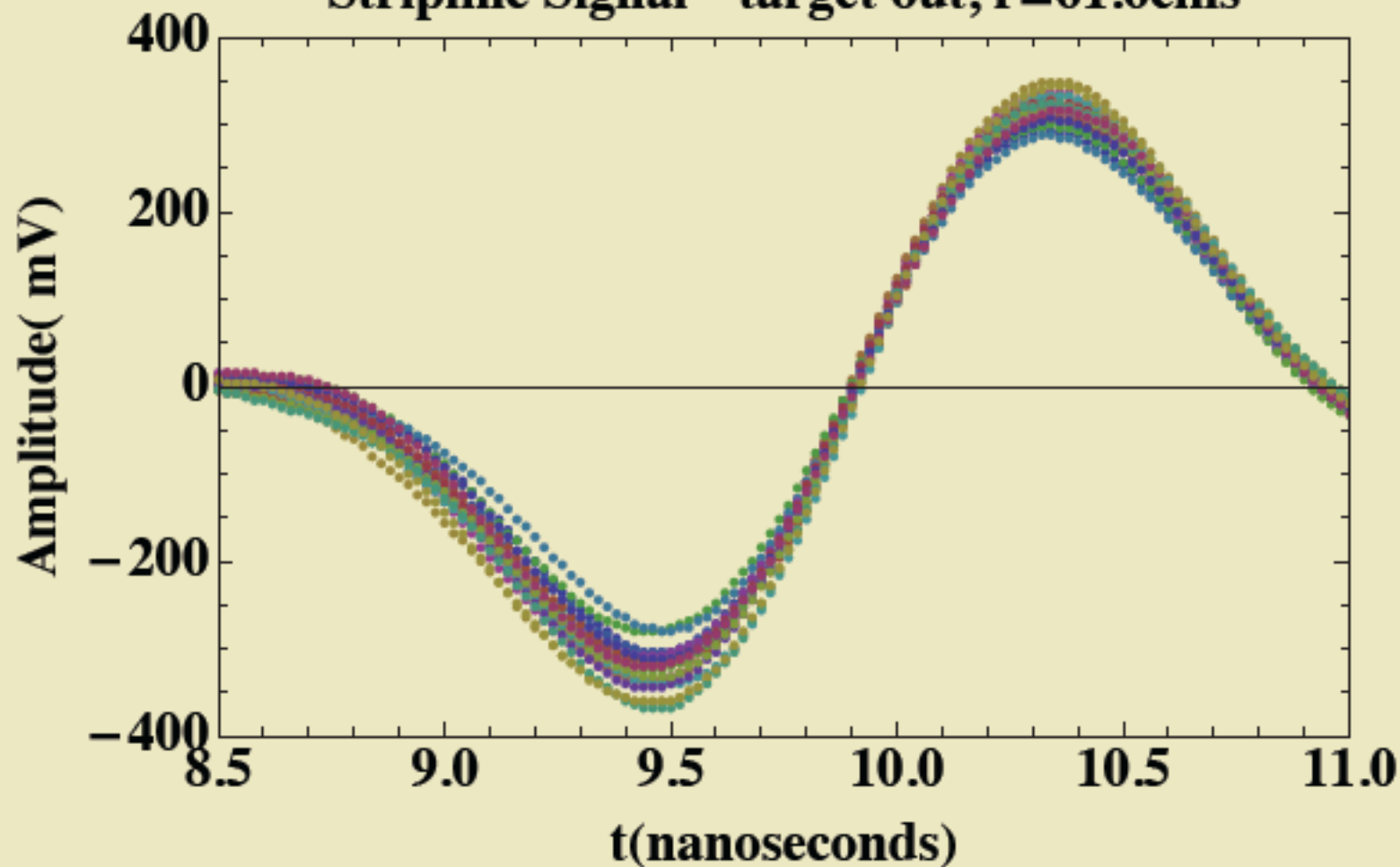
Stripline Signal– target out, r=61.6\text{cms}
