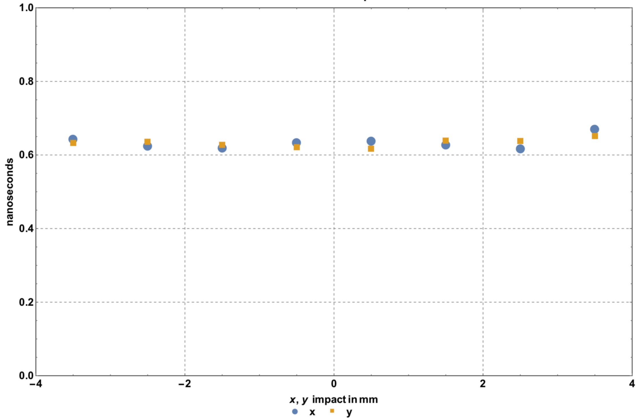
HFS Risettime vs Impact
