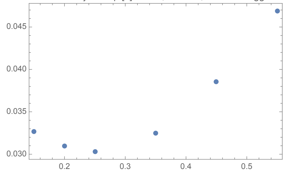
Difference time jitter/Sqrt[2]-linear,iorder=3,no CF vs. trigger level
