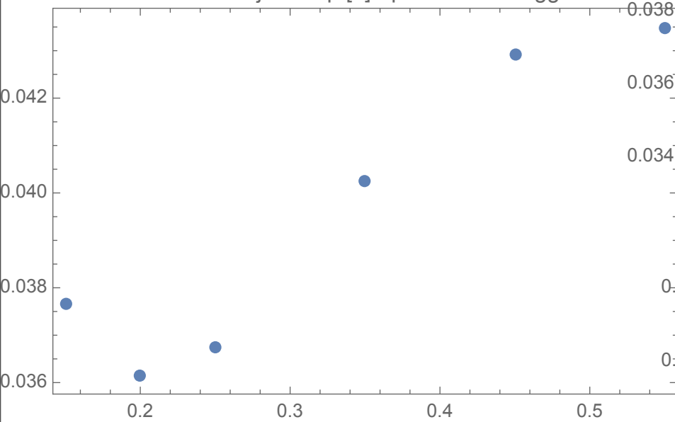
Difference time jitter/Sqrt[2]–quadratic vs. trigger level
