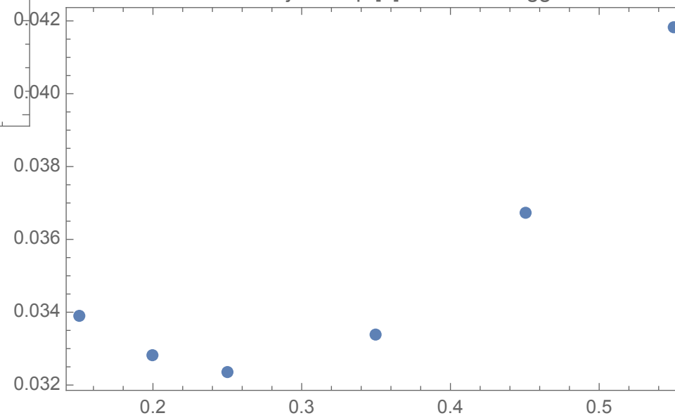
Difference time jitter/Sqrt[2]–linear vs. trigger level
