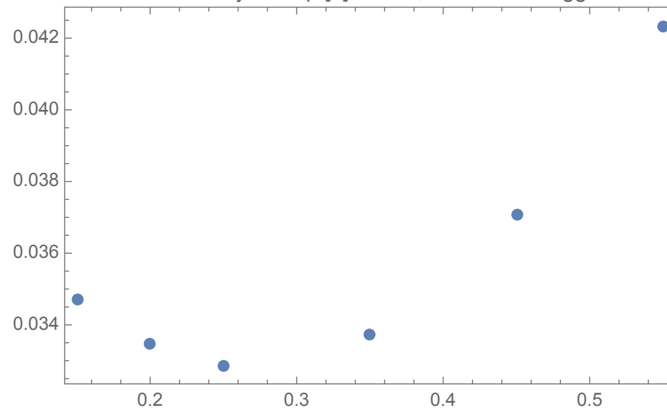
Difference time jitter/Sqrt[2]–linear,iorder=3 vs. trigger level
