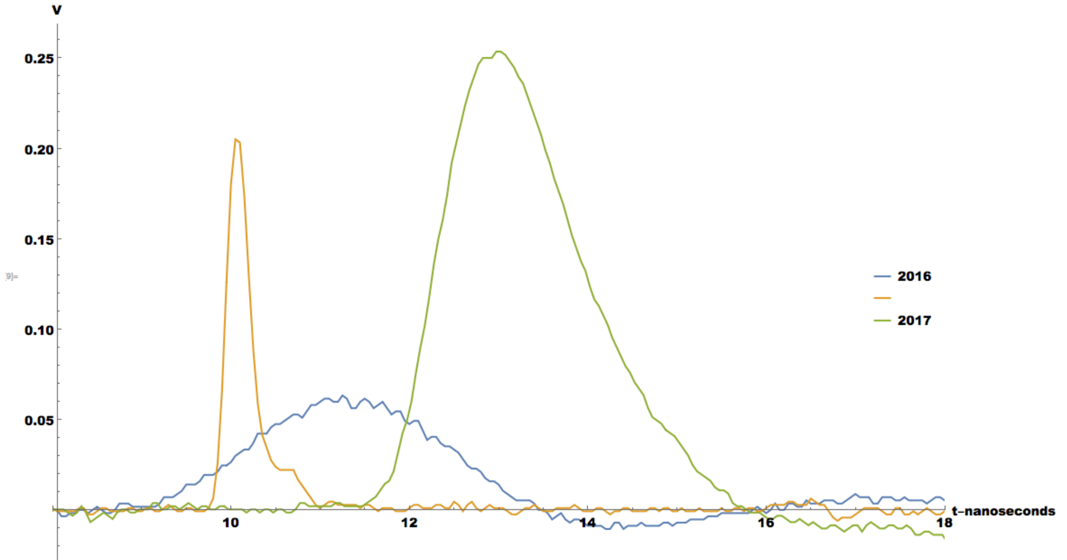
HFS: Comparison of 2016 and 2017 performance
