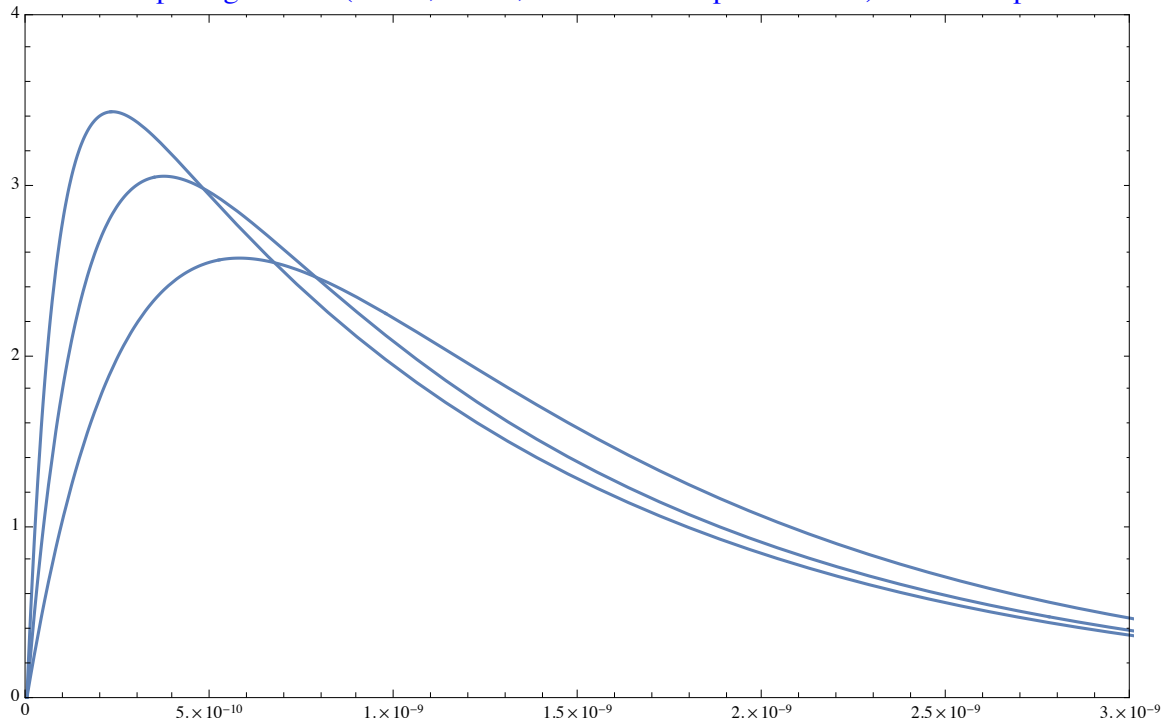
Output signal vs. t (2GHz, 1GHz, 0.5GHz Preamp bandwidth) for Cd=24pF
