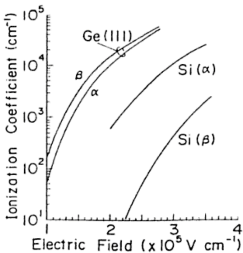
Figure 14 Impact ionization coefficients for silicon and germanium at 300 K. (From Ref. 8.)
