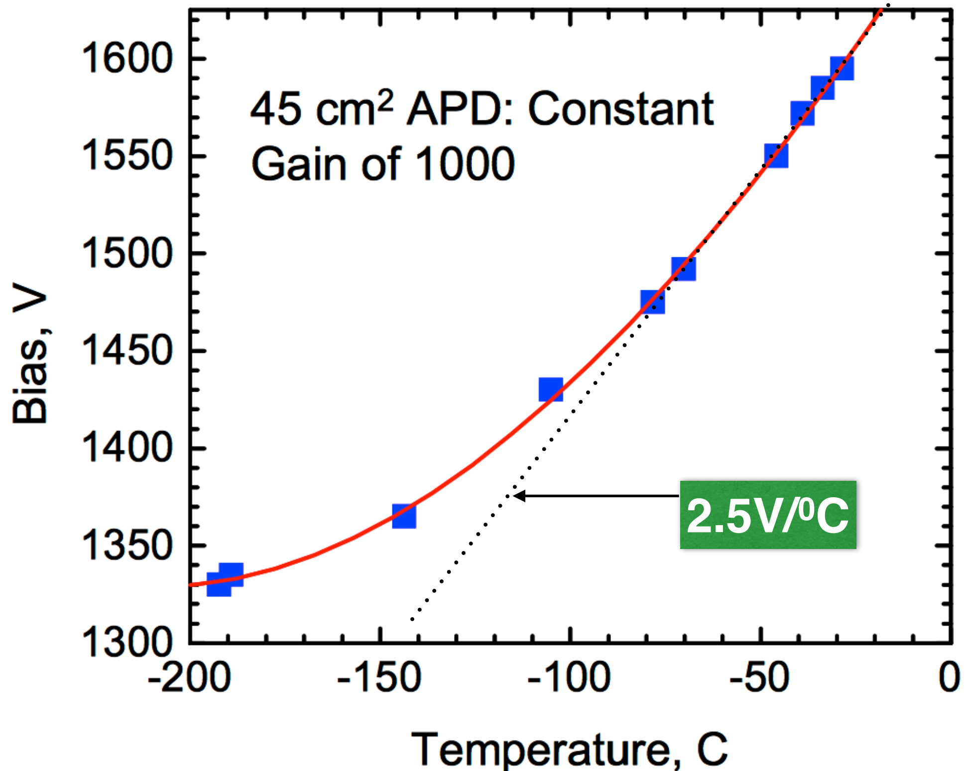
Figure 8. A constant gain of 1000 is maintained while 45 cm 2 APD is cooled to cryogenic temperature (77°K).
