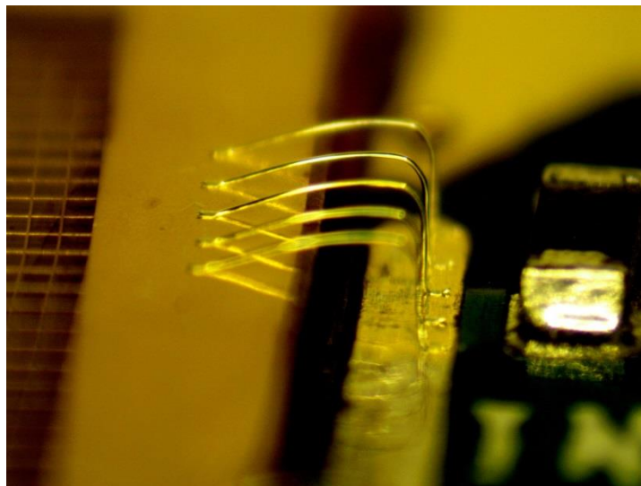
Wirebonded Mesh Contact to Amplifier Input
