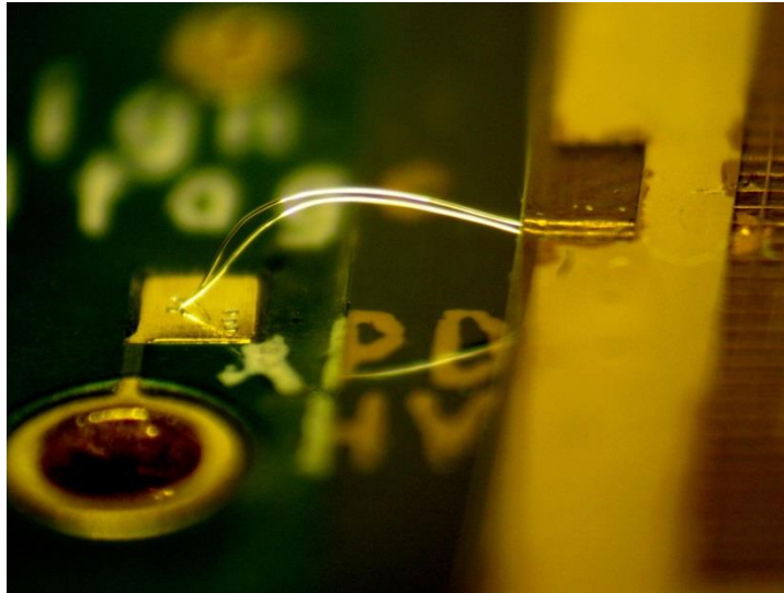
HV Wirebonded Top Contact
