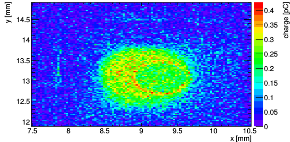
IR at 1600V
