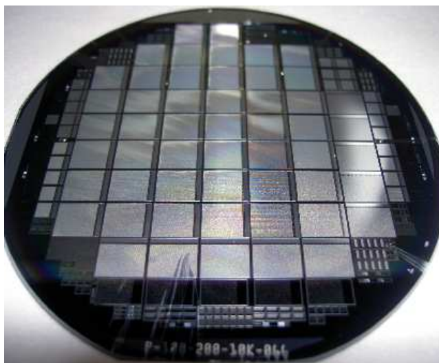
Figure 71. Four-inch wafer processed for the FP420 project. This has 32 3E, 6 4E and 6 2E ATLAS pixel readout compatible devices and several test structures. The 250 micron substrate is 12\text{ k}\Omega\text{ cm} p-type.
