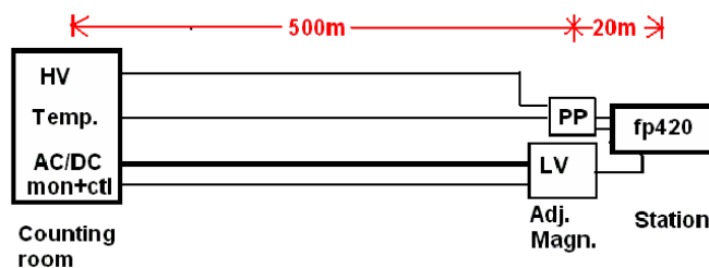
Figure 96. Overview of the Wiener Solution 2, based on the Maraton modules next to the cryostat. “Station” indicates the FP420 cryostat and “Adj. Magn.” the magnets adjacent to the FP420 cryostat. “PP” is a patch panel.
