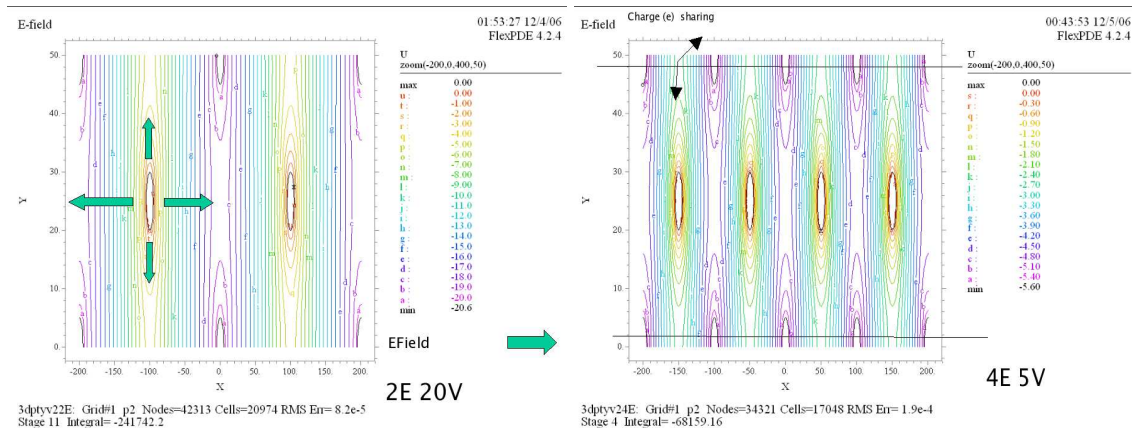
Figure 70. Equipotentials in a 2E and 4E 3D detector. Pixel size is 50\text{ }\mu\text{m} (Y) by 400\text{ }\mu\text{m} (X). The bias is 20 V and 5 V for the 2E and 4E devices respectively. The direction of the electric field is indicated. The n-electrodes are at the centre. A maximum field of 1\text{ V}/\mu\text{m} occurs at 24 V and 14 V in a 2E and 4E device respectively.
