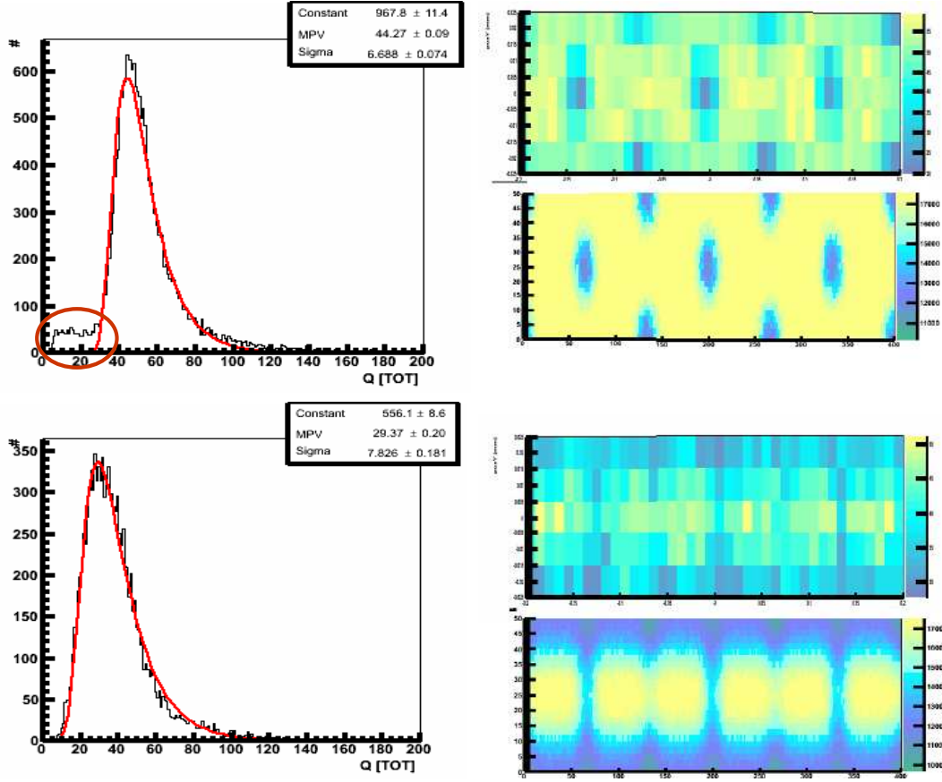
Figure 73. Left: Pulse height spectrum for 100 GeV/c pions incident perpendicularly (top) and at a 15° angle (bottom) on a 3E-3D detector biased at 20 V. One Q[TOT] ADC count is 600 electrons. The threshold was 3200 electrons. The tracking efficiencies are 95.9% and 99.9% respectively. This takes into account the partial response of the central part of the electrodes. Right: Simulations (bottom) are in good agreement with the experimental results (top) [M. Mathes, Bonn].
