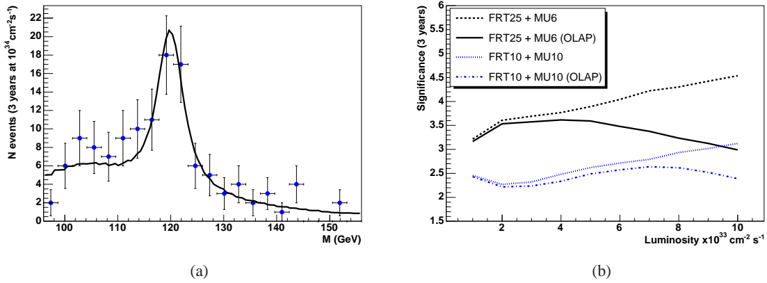
Figure 21. (a) Typical mass fit for the 120 GeV/c 2 MSSM h \rightarrow b\bar{b} for 3 years of data taking at 10^{34} \text{ cm}^{-2} \text{ s}^{-1} after removing the overlap background contribution completely with improved timing detectors. The significance is 5\sigma for these data. (b) Significance of the measurement of the 120 GeV/c 2 MSSM Higgs boson versus luminosity, for two different combinations of muon — MU6, MU10 — and jet-rate — FRT25, FRT10 — triggers, see section 3.1, and with an improved (baseline) FP420 timing design (OLAP labels).
