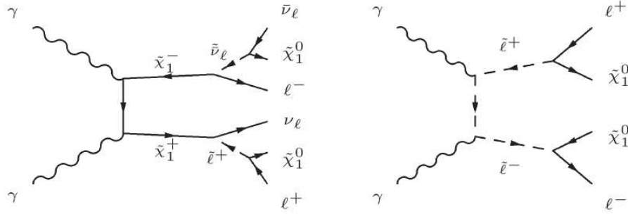
Figure 10. Relevant Feynman diagrams for SUSY pair production with leptons in the final state: chargedino disintegration in a charged/neutral scalar and a neutral/charged fermion (left); slepton disintegration (right) [12].
