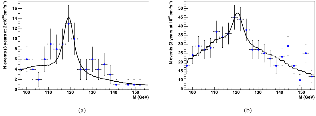
Figure 20. Typical mass fits for the 120 GeV/c 2 MSSM h \rightarrow b\bar{b} , with the L1 trigger and analysis cuts discussed in the text, for 3 years of data taking at 2 \times 10^{33} \text{ cm}^{-2} \text{ s}^{-1} (60 fb -1 , 3.5 \sigma , left plot) and at 10^{34} \text{ cm}^{-2} \text{ s}^{-1} (300 fb -1 , 3 \sigma , right plot).
