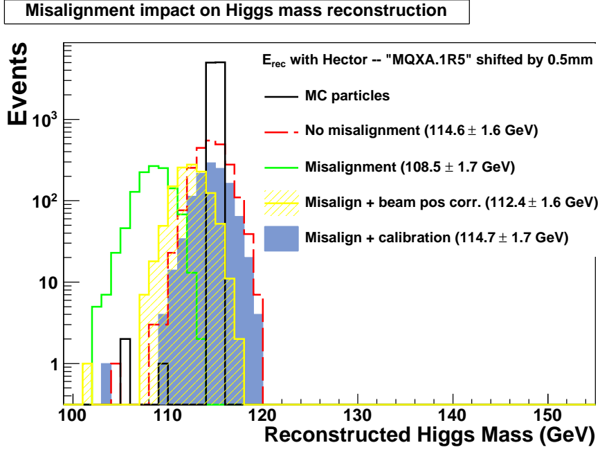
Figure 125. Illustration of the effect on the missing mass reconstruction due to a misalignment of LHC quadrupoles. In this example a quadrupole (MQXA1R5) has been misaligned by 500\ \mu\text{m} . Data from BPMs cannot fully recover the mass shift, while the exclusive dimuon calibration recovers it fully, and the resolution is not affected as long as the misalignment is stable [61].
