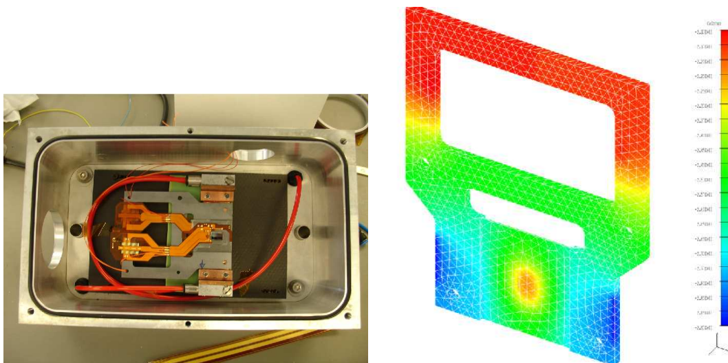
Figure 83. Left: A thermal model blade with the silicon resistors as described in the text. Right: Finite element analysis of the thermal properties of a blade.
