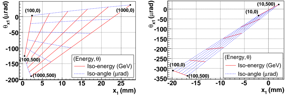
Figure 27. Chromaticity grids: iso-energy and iso-angle lines for 220 m (left) and 420 m (right) detectors at IP5, beam 1 computed with HECTOR. The vertical axis \theta_{x1} is the angle of the scattered proton relative to the beam at 220 or 420 m, and the horizontal axis x_1 is the horizontal displacement of the scattered proton relative to the beam. The solid red lines are iso-energy lines, ranging from proton energy loss 0 GeV to 1000 GeV in steps of 200 GeV at 220 m, and from 0 GeV to 100 GeV in steps of 20 GeV at 420 m. The dotted blue lines are lines of constant proton emission angle at the interaction point, and range from 0 \mu\text{rad} to 500 \mu\text{rad} in steps of 100 \mu\text{rad} .
