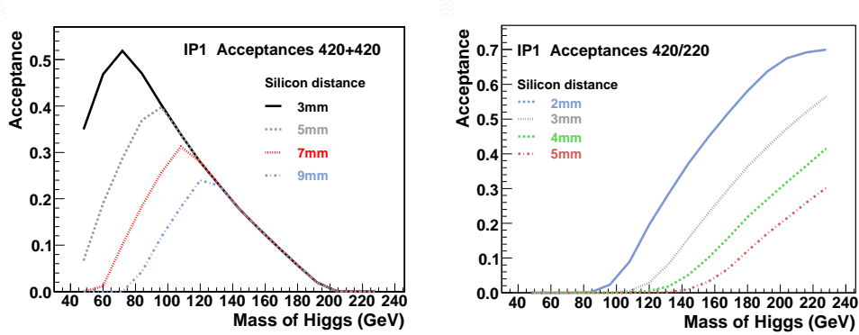
Figure 28. Acceptance as a function of centrally produced mass for (left) 420 + 420 m proton tags for the silicon detector active edge positioned at different distances from the beam; (right) for 220 + 420 m proton tags with the 420 m silicon at 5 mm from the beam and the 220 m at different distances from the beam. The small upward deviation at high mass for the 2 mm silicon positions, show the additional acceptance from 220 + 220 m coincidences.
