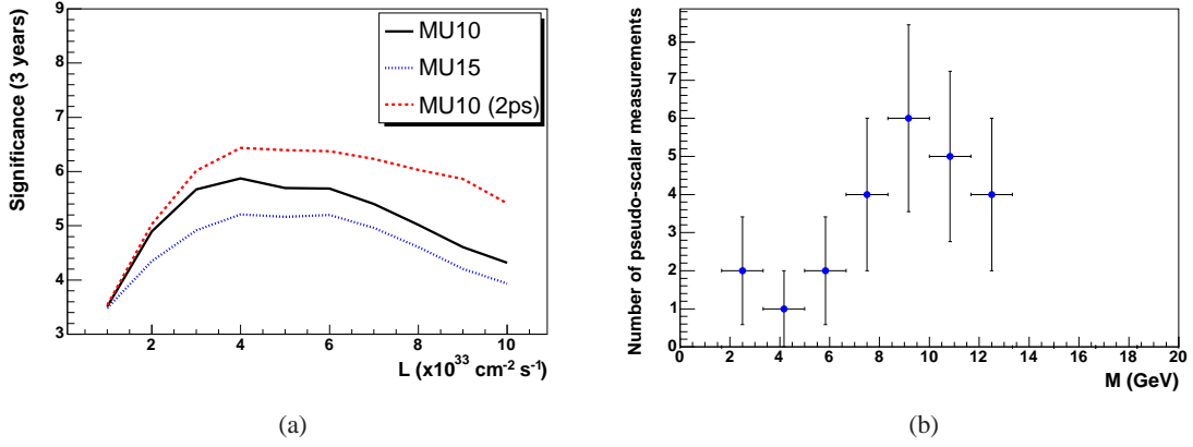
Figure 7. (a) The significance of observation of h \rightarrow aa \rightarrow 4\tau using a muon p_T trigger threshold of 10 GeV/c (or 15 GeV/c) for three years of data taking at ATLAS and CMS. Also shown is the increase in the significance due to a factor of five improvement in background rejection from a 2 ps proton time-of-flight measurement, see sections 3 and 10, or a comparable gain across all of the rejection variables [27]. (b) A typical a mass measurement for 150 \text{ fb}^{-1} of data.
