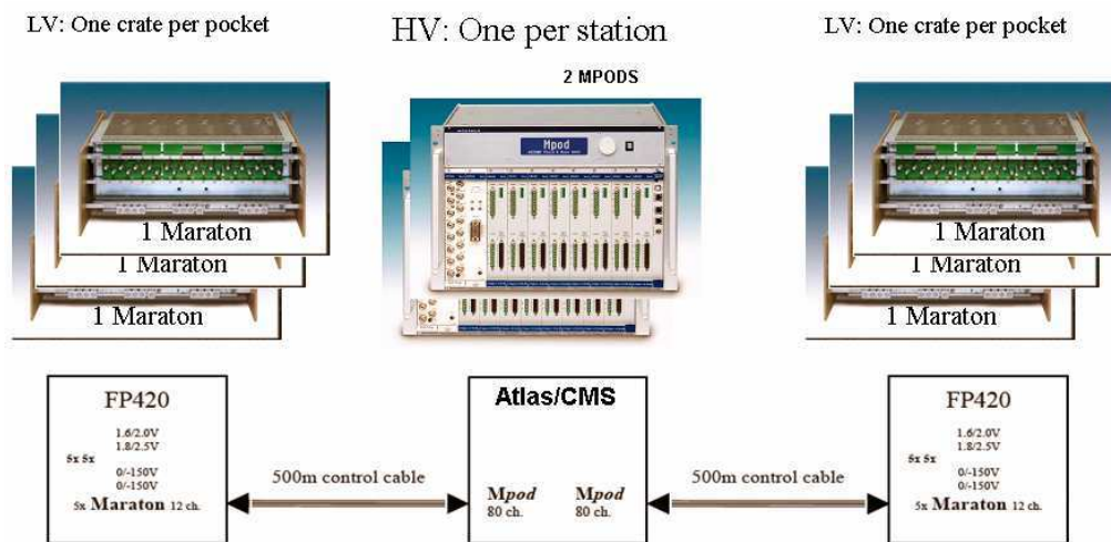
Figure 97. Low-voltage Wiener Maraton supplies in the tunnel. High-voltage MPOD type supplies are located in the counting room. The Wiener Maraton system is qualified for the radiation environment expected in the tunnel under the magnets near the FP420 cryostat. The illustration shows the setup for either ATLAS or CMS. “Station” indicates the FP420 cryostat.
