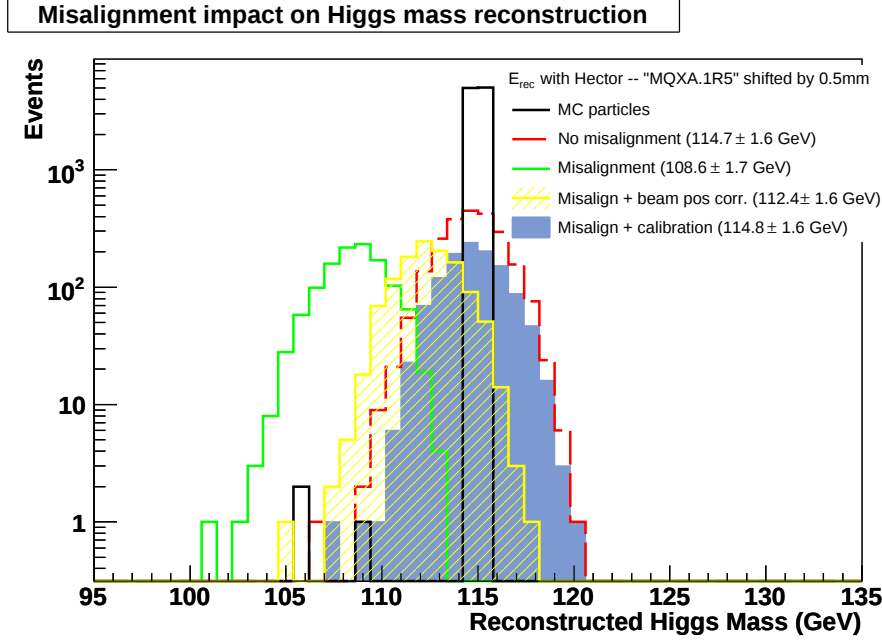
Fig. 126: Illustration of the effect on the missing mass reconstruction due to a misalignment of LHC quadrupoles. In this example a quadrupole (MQXA1R5) has been misaligned by 500 \mu\text{m} . Data from BPMs cannot fully recover the mass shift, while the exclusive dimuon calibration recovers it fully, and the resolution is not affected as long as the misalignment is stable [60].
