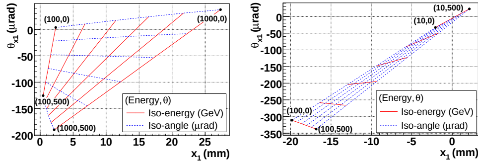
Fig. 27: Chromaticity grids: iso-energy and iso-angle lines for 220 m (left) and 420 m (right) detectors at IP5, beam 1 computed with HECTOR. The vertical axis \theta_{x1} is the angle of the scattered proton relative to the beam at 220 or 420 m, and the horizontal axis x_1 is the horizontal displacement of the scattered proton relative to the beam. The solid lines are iso-energy lines, ranging from proton energy loss 0 GeV to 1000 GeV in steps of 200 GeV at 220 m, and from 0 GeV to 100 GeV in steps of 20 GeV at 420 m. The dotted lines are lines of constant proton emission angle at the interaction point, and range from 0 \mu\text{rad} to 500 \mu\text{rad} in steps of 100 \mu\text{rad} .
