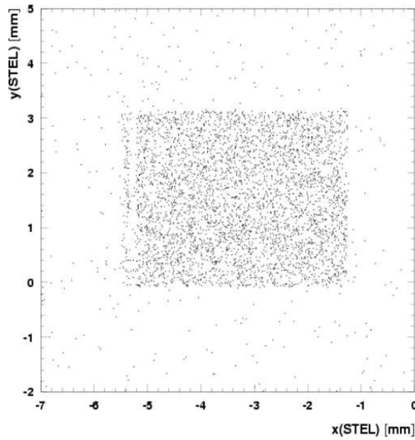
Fig. 66: Two-dimensional efficiency map of a fully operational 3D detector. A point is plotted with respect to the position (x,y) predicted by a telescope, with a precision of 4\text{ }\mu\text{m} as a valid track and a hit was recorded by a 3D detector. The inefficient band near the lower x-edge was caused by the detector's bonding pads. The upper and lower y edges were used for active edge measurements and showed a device sensitivity up to 4 microns of the physical edge.
