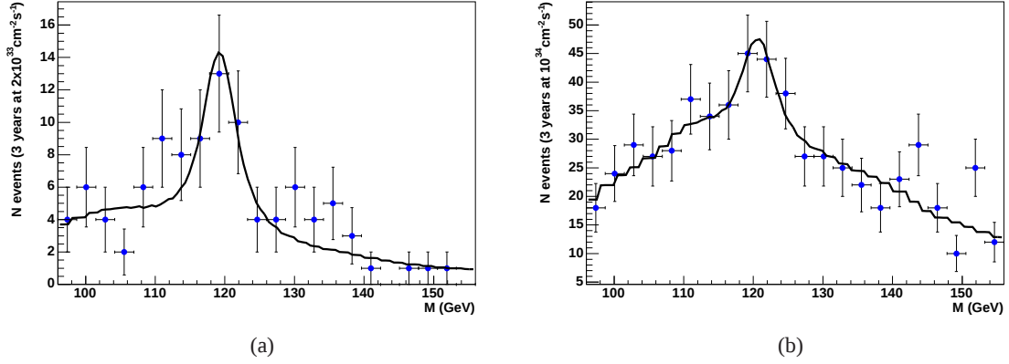
Fig. 20: Typical mass fits for the 120 GeV/c 2 MSSM h \rightarrow b\bar{b} , with the L1 trigger and analysis cuts discussed in the text, for 3 years of data taking at 2 \times 10^{33} \text{ cm}^{-2} \text{ s}^{-1} (60 fb -1 3.5 \sigma , left plot) and at 10^{34} \text{ cm}^{-2} \text{ s}^{-1} (300 fb -1 , 3 \sigma , right plot).
