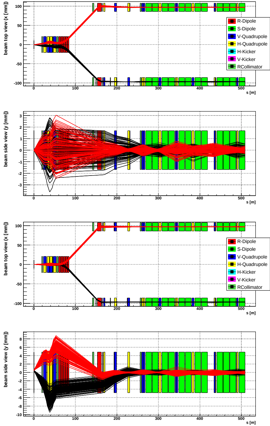
Fig. 124: Beam particle paths calculated by HECTOR [60], around CMS (top two figures) and ATLAS (bottom two figures). The beam line has been artificially straightened through the dipole region z > 250 m.
