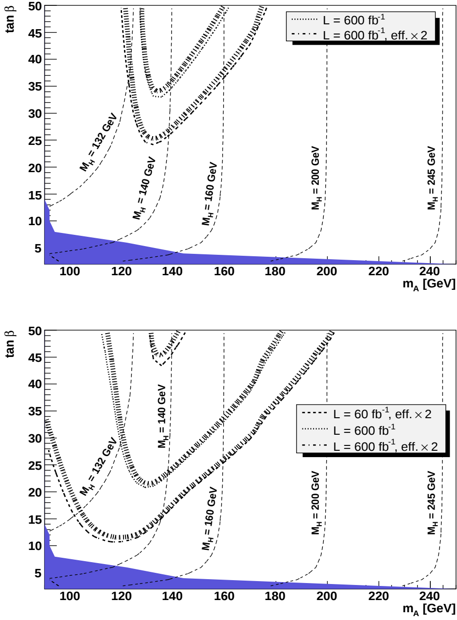
Fig. 6: 5 \sigma discovery contours (upper plot) and contours of 3 \sigma statistical significance (lower plot) for the H \rightarrow \tau^+\tau^- channel in CEP in the m_A - \tan\beta plane of the MSSM within the M_h^{max} benchmark scenario (with \mu = +200\text{GeV} ) for different luminosities. The values of the mass of the heavier CP-even Higgs boson, M_H , are indicated by contour lines. No pile-up background assumed. The dark shaded (blue) region corresponds to the parameter region that is excluded by the LEP Higgs boson searches.
