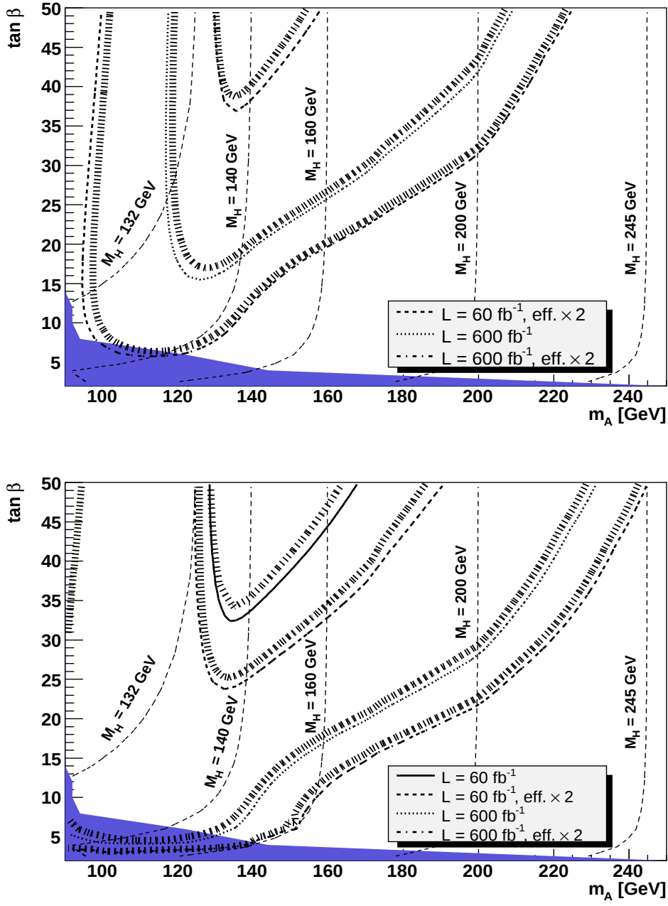
Fig. 5: 5 \sigma discovery contours (upper plot) and contours of 3 \sigma statistical significance (lower plot) for the CEP H \rightarrow b\bar{b} channel in the M_A - \tan\beta plane of the MSSM within the M_h^{max} benchmark scenario (with \mu = +200\text{GeV} ) for different luminosity scenarios as described in the text [19]. The values of the mass of the heavier CP-even Higgs boson, M_H , are indicated by contour lines. No pile-up background assumed. The dark shaded (blue) region corresponds to the parameter region that is excluded by the LEP Higgs searches [41, 42].
