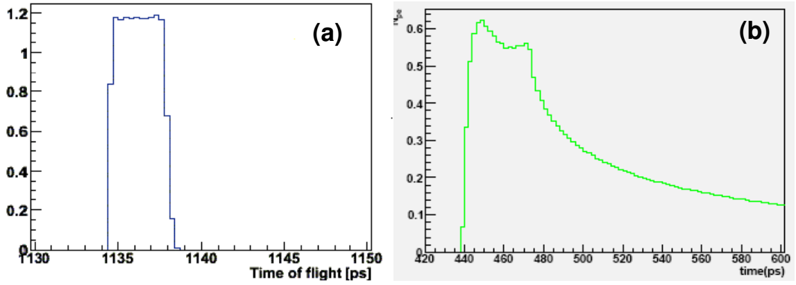
Fig. 117: Simulated time of arrival of Čerenkov photons at the MCP-PMT photocathode for (a) GASTOF (b) QUARTIC.
