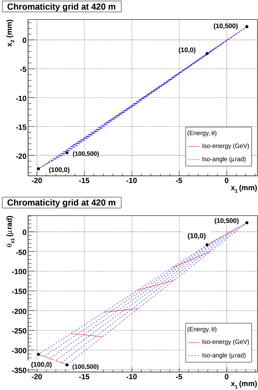
Fig. 125: Chromaticity grids: iso-energy loss and iso-production angle lines, from 10 GeV to 100 GeV and 0 to 500 \mu\text{rad} [60].
