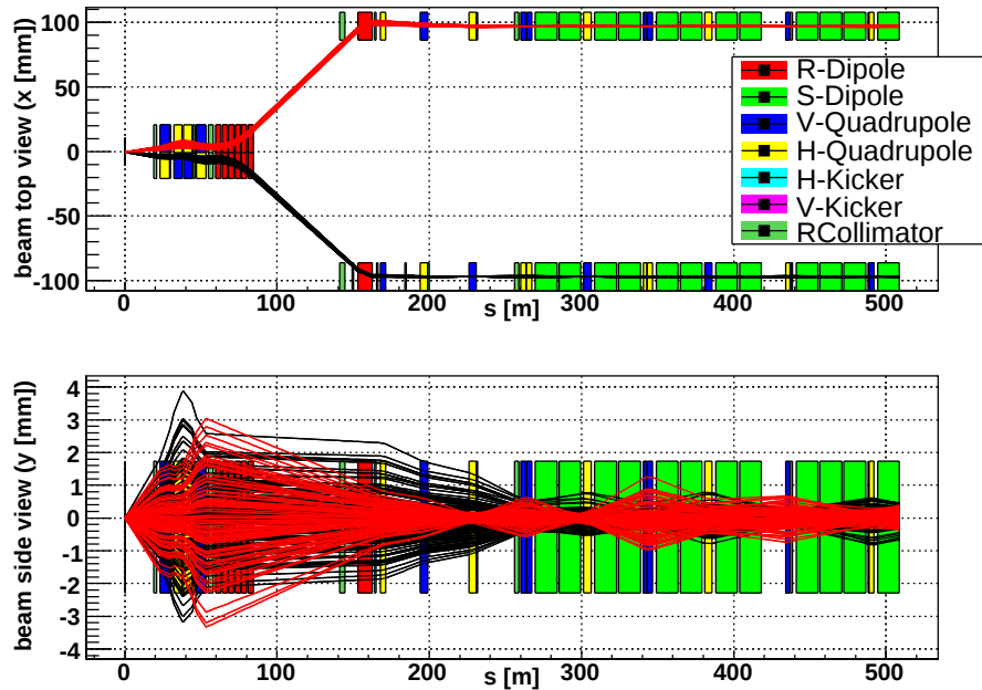
Fig. 23: Schematic plan view and side view of the beamline at IP5 (CMS); the IP1 configuration (ATLAS) is similar except that the kicker magnets are vertical (see also Fig. 124) [60]. The horizontal curvature of the beamline has been straightened out for purposes of simplification here.
