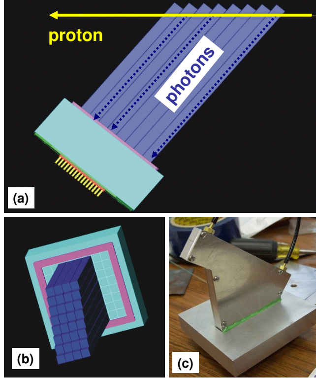
Fig. 116: Conceptual drawings of a QUARTIC detector, (a) showing the proton passing through eight bars of one row in x providing eight measurements of the proton time (b) showing the 4 \times 8 layout of QUARTIC bars (c) A photograph of the prototype detector used in the June 2008 CERN test beam.
