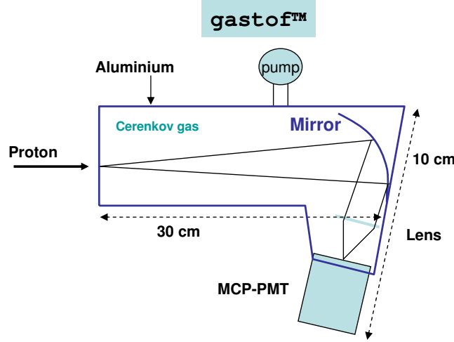
Fig. 115: Schematic of GASTOF, a gas-based Čerenkov counter proposed by Louvain-la-Neuve, as described in the text.
