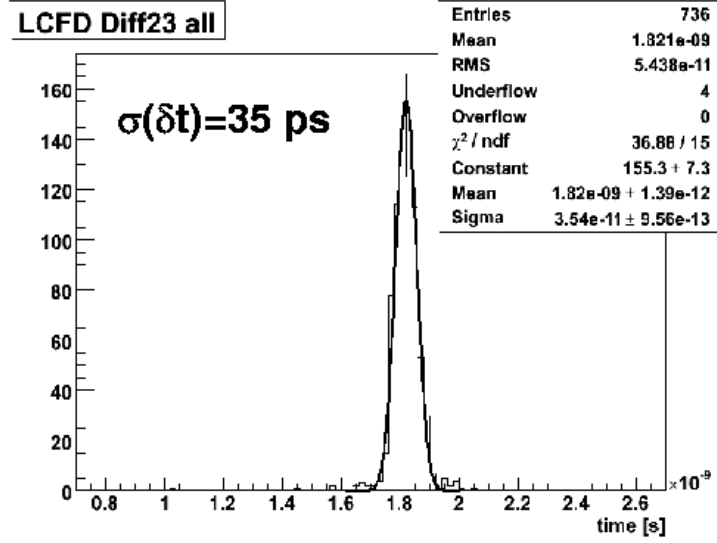
Fig. 118: The time difference between the first (G1) and second generation (G2) GASTOF prototype detectors from the March 2007 test beam.
