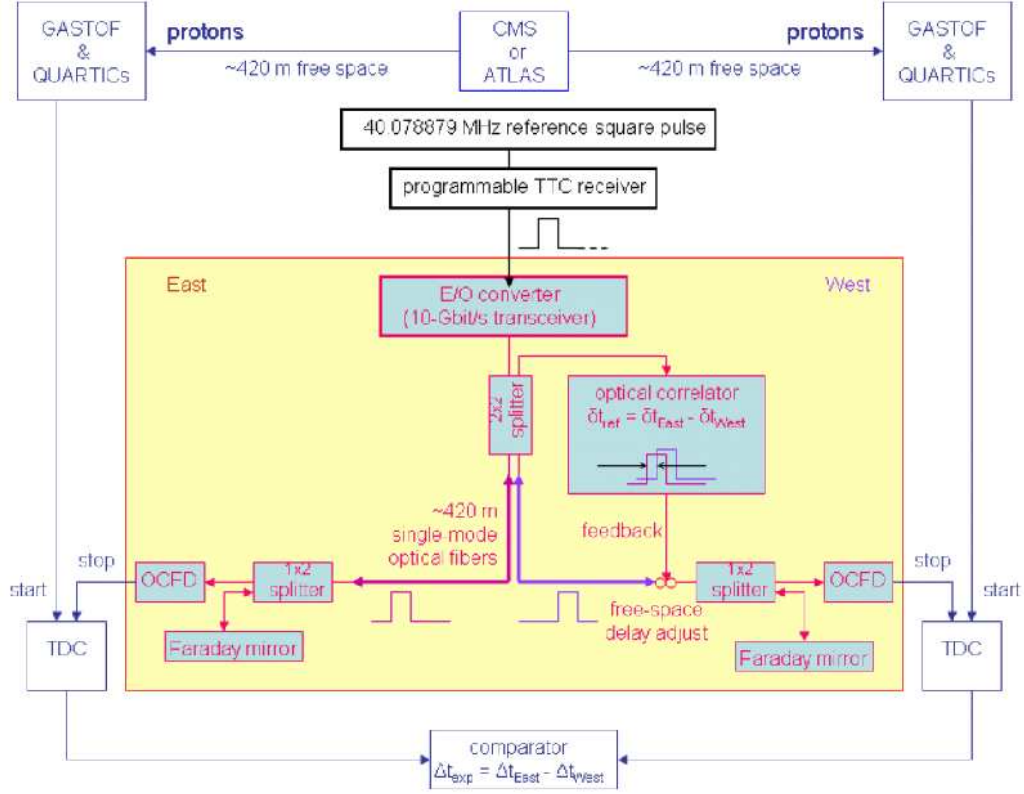
Fig. 120: A schematic of the reference time system. Components labeled in black are expected to come from CERN TTC system, components labeled in blue are associated with the ToF detectors, and the components in red (highlighted in the yellow box) are the optical components related to the reference timing system.
