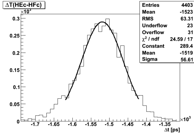
Fig. 119: The time difference between two 90 mm long QUARTIC bars as described in text.
