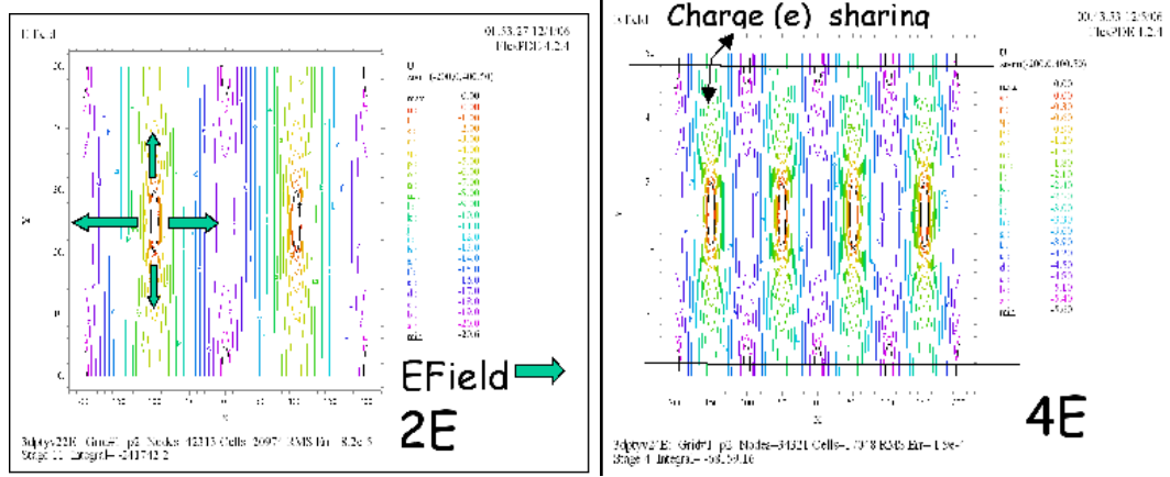
Fig. 70: Equipotentials in a 2E and 4E 3D detector. Pixel size is 50\ \mu\text{m} (Y) by 400\ \mu\text{m} (X). The bias is 20 V and 5 V for the 2E and 4E devices respectively. The direction of the electric field is indicated. The n-electrodes are at the centre. A maximum field of 1\ \text{V}/\mu\text{m} occurs at 24 V and 14 V in a 2E and 4E device respectively.
