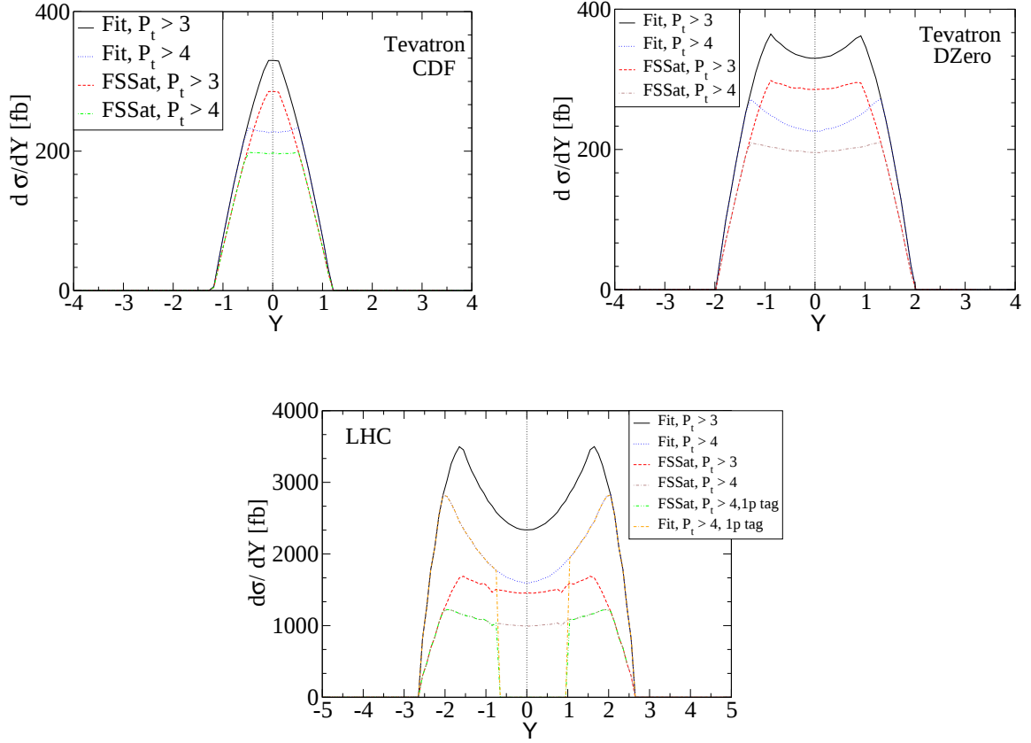
Figure 8: The \Upsilon rapidity distribution after cuts at the Tevatron (top) and LHC (bottom) using the FSSat dipole model and the the parameterization the photoproduction data described in the text.
